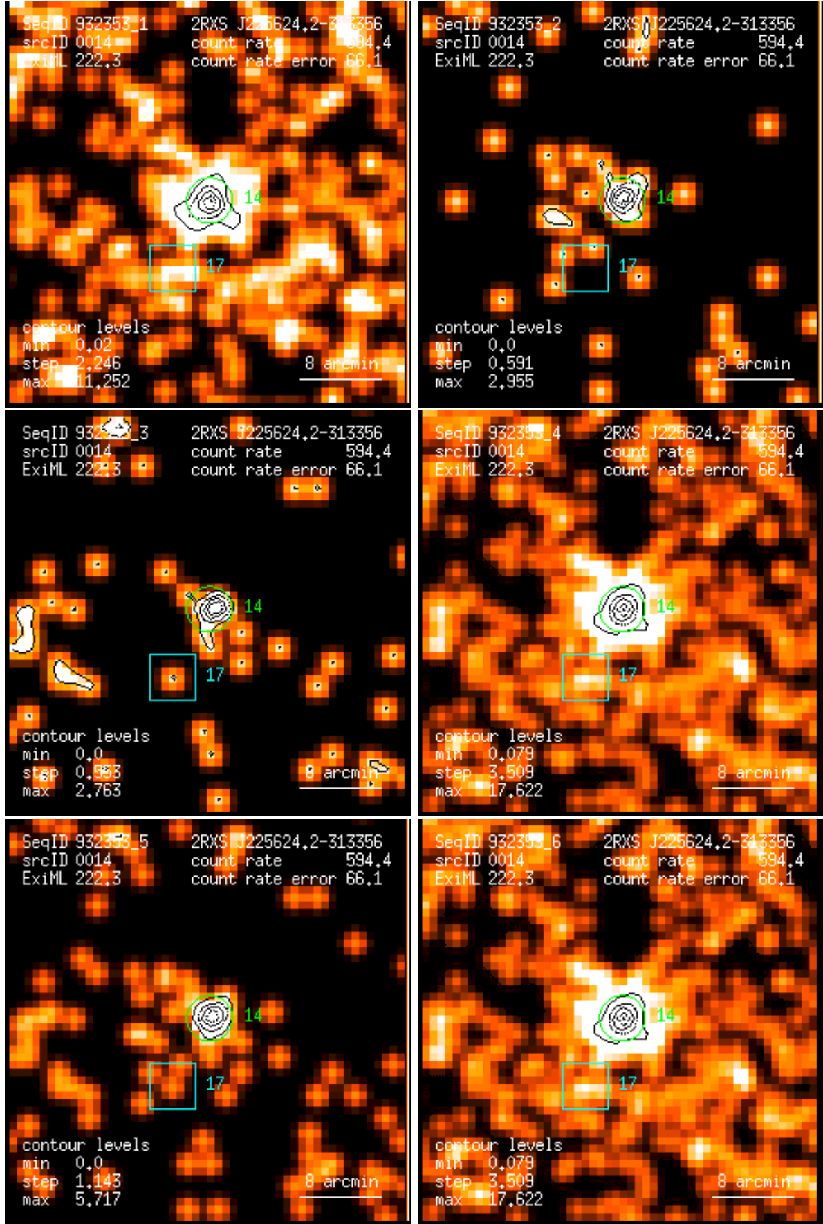
Figure 14: RASS 932353: detection 0014: band rate images, Gaussian filter: (1) PSPC channels 11 – 41, (2) 52 – 90, (3) 91 – 201, (4) 11 – 235, (5) 52 – 201, (6) 11 – 201. Broad band rates in counts/ks. Band rate contour levels in counts/ks/arcmin 2 .
