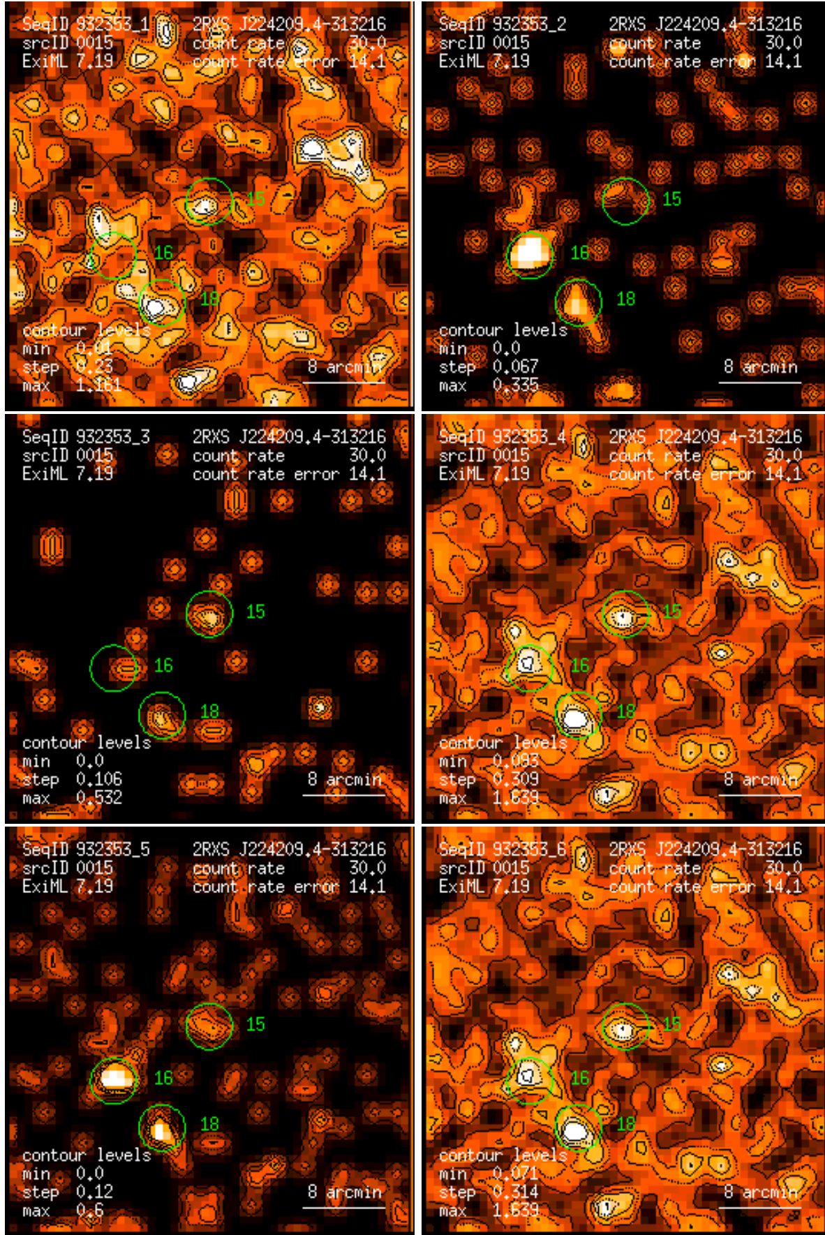
Figure 15: RASS 932353: detection 0015: band rate images, Gaussian filter: (1) PSPC channels 11 – 41, (2) 52 – 90, (3) 91 – 201, (4) 11 – 235, (5) 52 – 201, (6) 11 – 201. Broad band rates in counts/ks. Band rate contour levels in counts/ks/arcmin 2 .
