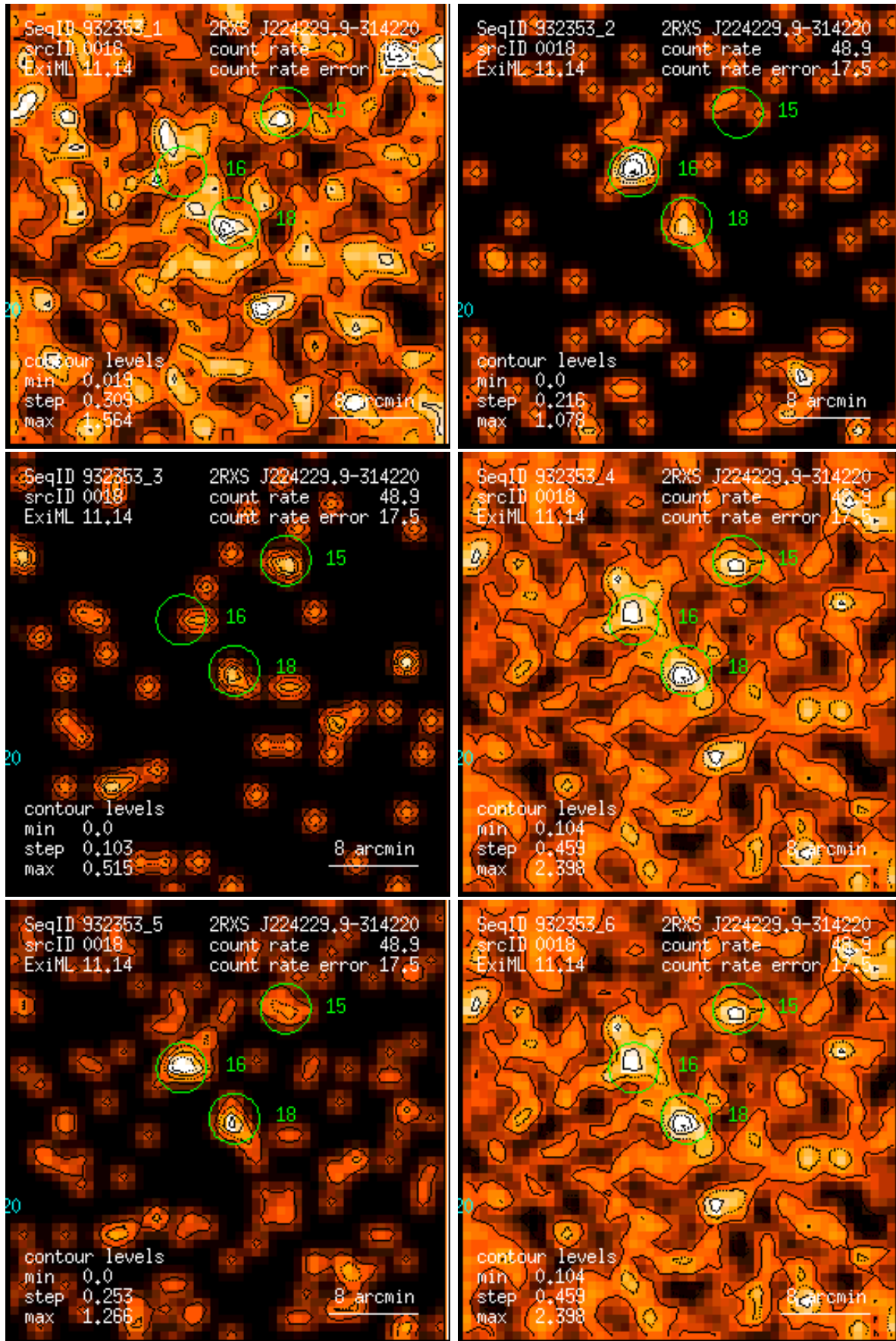
Figure 18: RASS 932353: detection 0018: band rate images, Gaussian filter: (1) PSPC channels 11 – 41, (2) 52 – 90, (3) 91 – 201, (4) 11 – 235, (5) 52 – 201, (6) 11 – 201. Broad band rates in counts/ks. Band rate contour levels in counts/ks/arcmin 2 .
