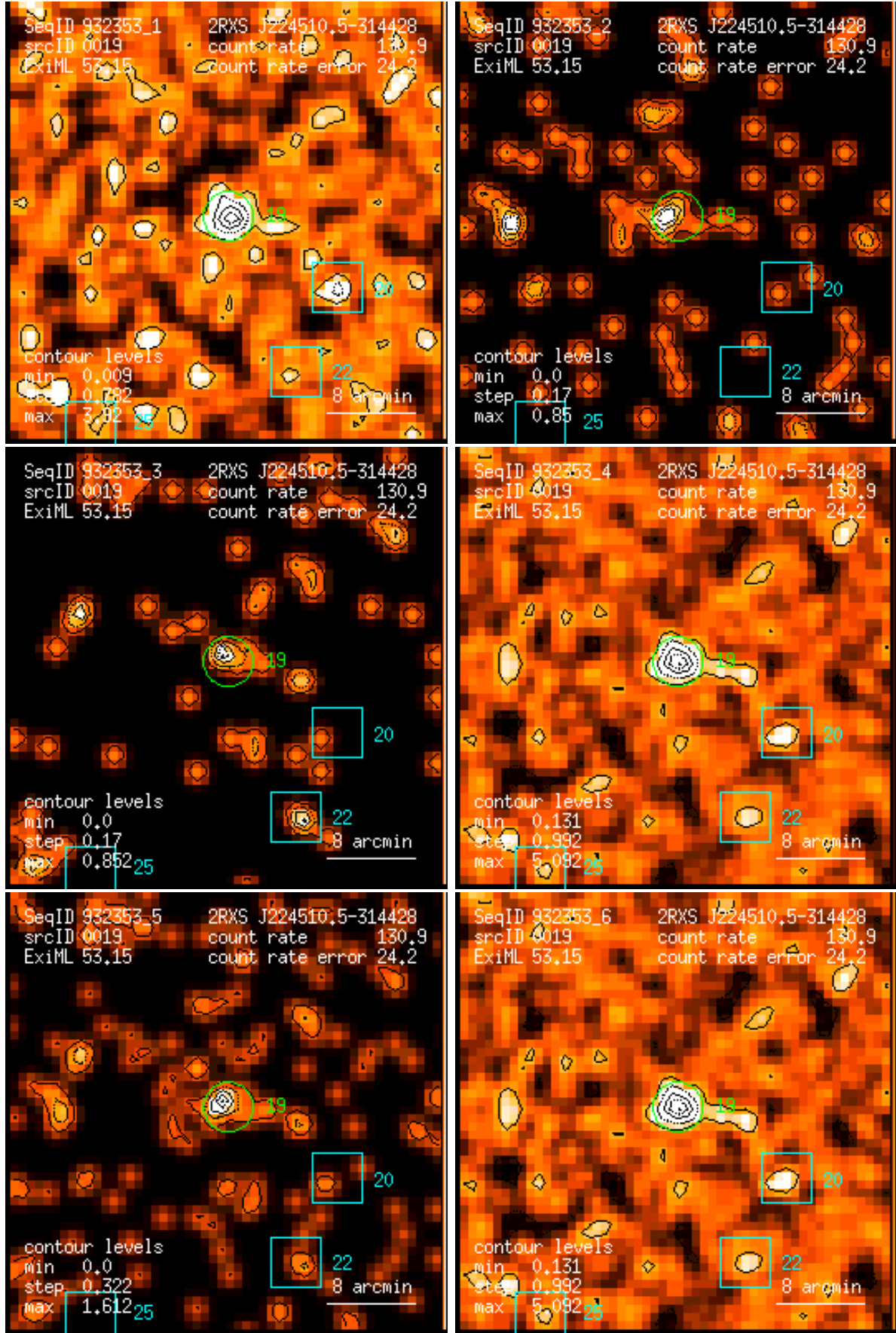
Figure 19: RASS 932353: detection 0019: band rate images, Gaussian filter: (1) PSPC channels 11 – 41, (2) 52 – 90, (3) 91 – 201, (4) 11 – 235, (5) 52 – 201, (6) 11 – 201. Broad band rates in counts/ks. Band rate contour levels in counts/ks/arcmin 2 .
