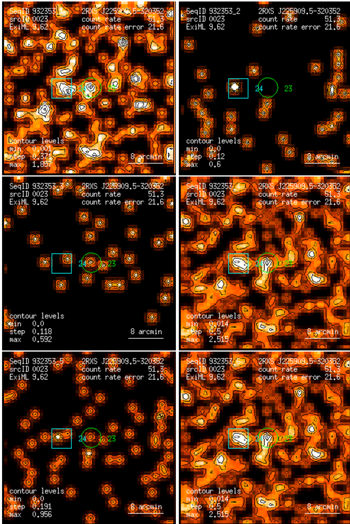
Figure 23: RASS 932353: detection 0023: band rate images, Gaussian filter: (1) PSPC channels 11 – 41, (2) 52 – 90, (3) 91 – 201, (4) 11 – 235, (5) 52 – 201, (6) 11 – 201. Broad band rates in counts/ks. Band rate contour levels in counts/ks/arcmin 2 .
