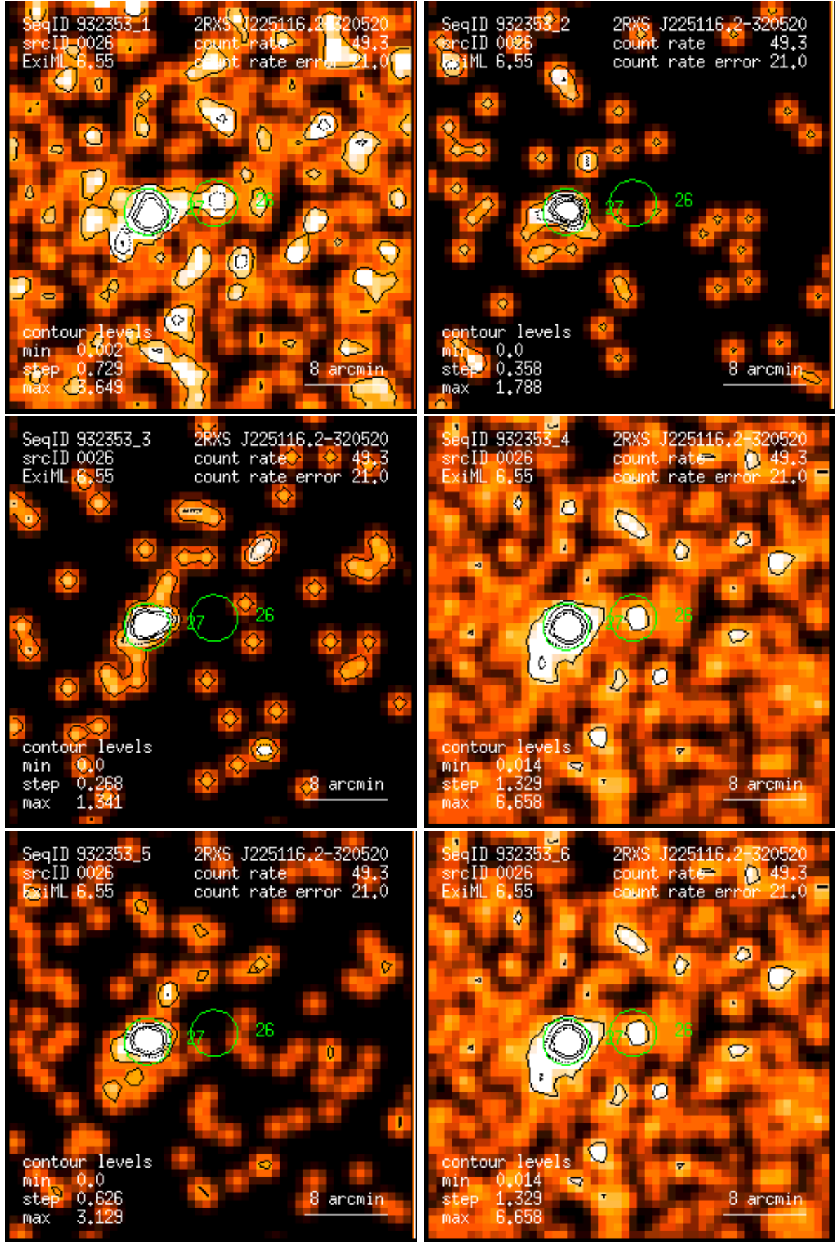
Figure 26: RASS 932353: detection 0026: band rate images, Gaussian filter: (1) PSPC channels 11 – 41, (2) 52 – 90, (3) 91 – 201, (4) 11 – 235, (5) 52 – 201, (6) 11 – 201. Broad band rates in counts/ks. Band rate contour levels in counts/ks/arcmin 2 .
