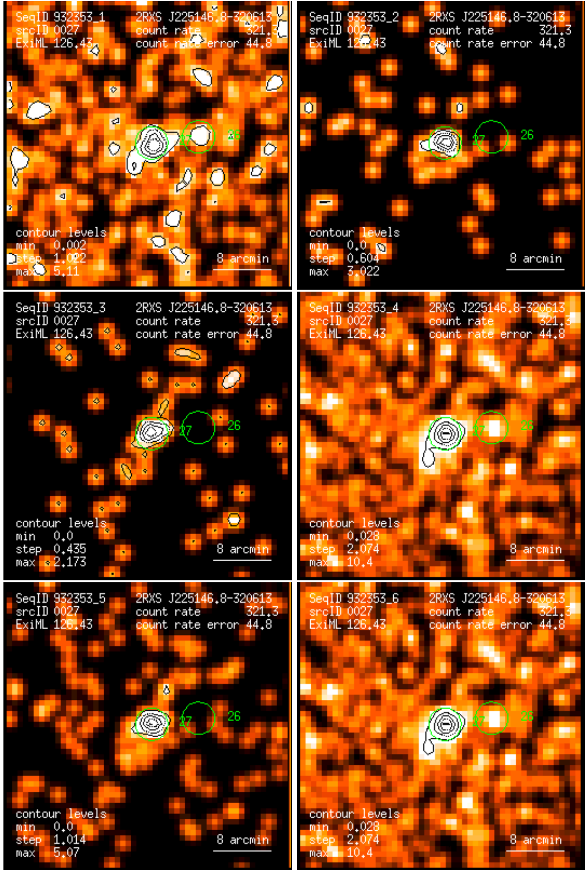
Figure 27: RASS 932353: detection 0027: band rate images, Gaussian filter: (1) PSPC channels 11 – 41, (2) 52 – 90, (3) 91 – 201, (4) 11 – 235, (5) 52 – 201, (6) 11 – 201. Broad band rates in counts/ks. Band rate contour levels in counts/ks/arcmin 2 .
