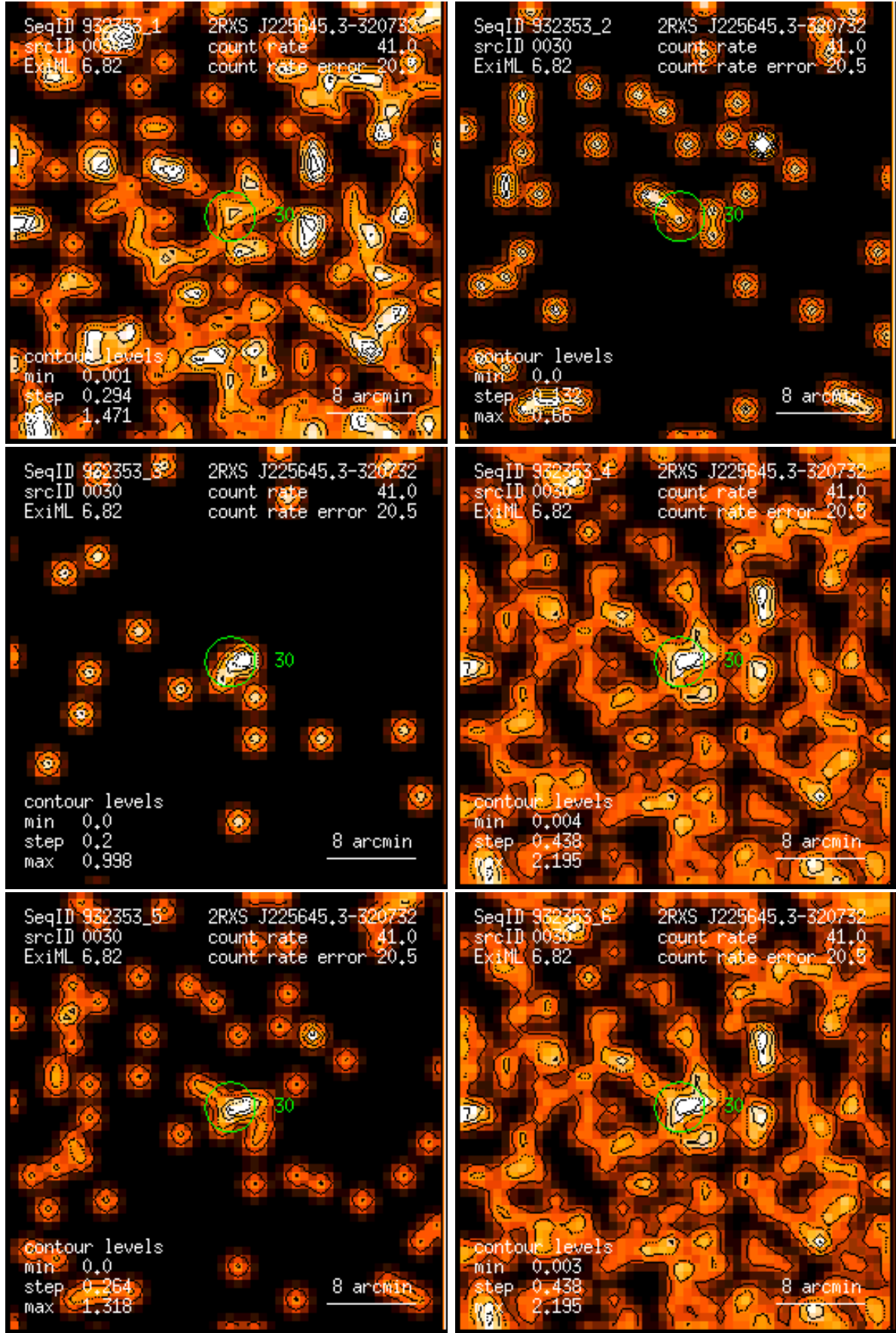
Figure 30: RASS 932353: detection 0030: band rate images, Gaussian filter: (1) PSPC channels 11 – 41, (2) 52 – 90, (3) 91 – 201, (4) 11 – 235, (5) 52 – 201, (6) 11 – 201. Broad band rates in counts/ks. Band rate contour levels in counts/ks/arcmin 2 .
