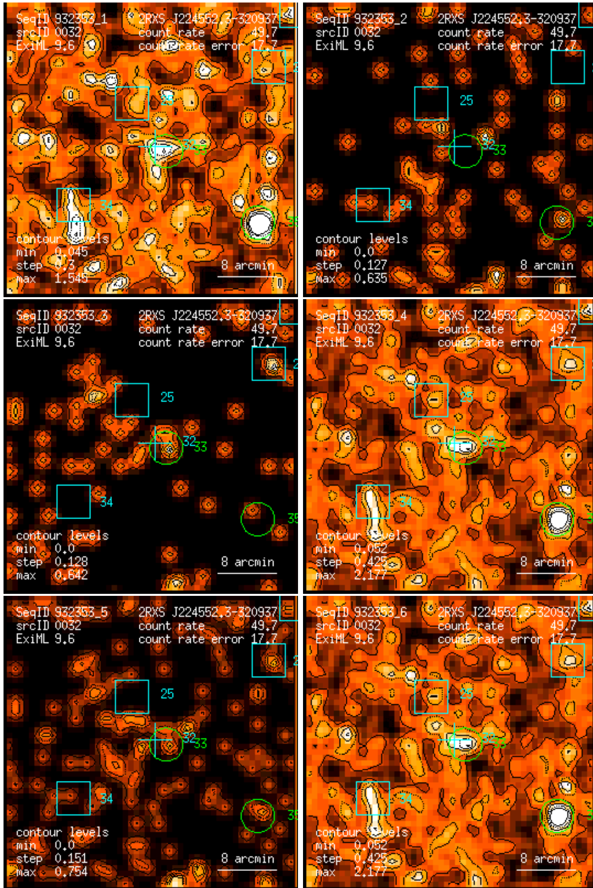
Figure 32: RASS 932353: detection 0032: band rate images, Gaussian filter: (1) PSPC channels 11 – 41, (2) 52 – 90, (3) 91 – 201, (4) 11 – 235, (5) 52 – 201, (6) 11 – 201. Broad band rates in counts/ks. Band rate contour levels in counts/ks/arcmin 2 .
