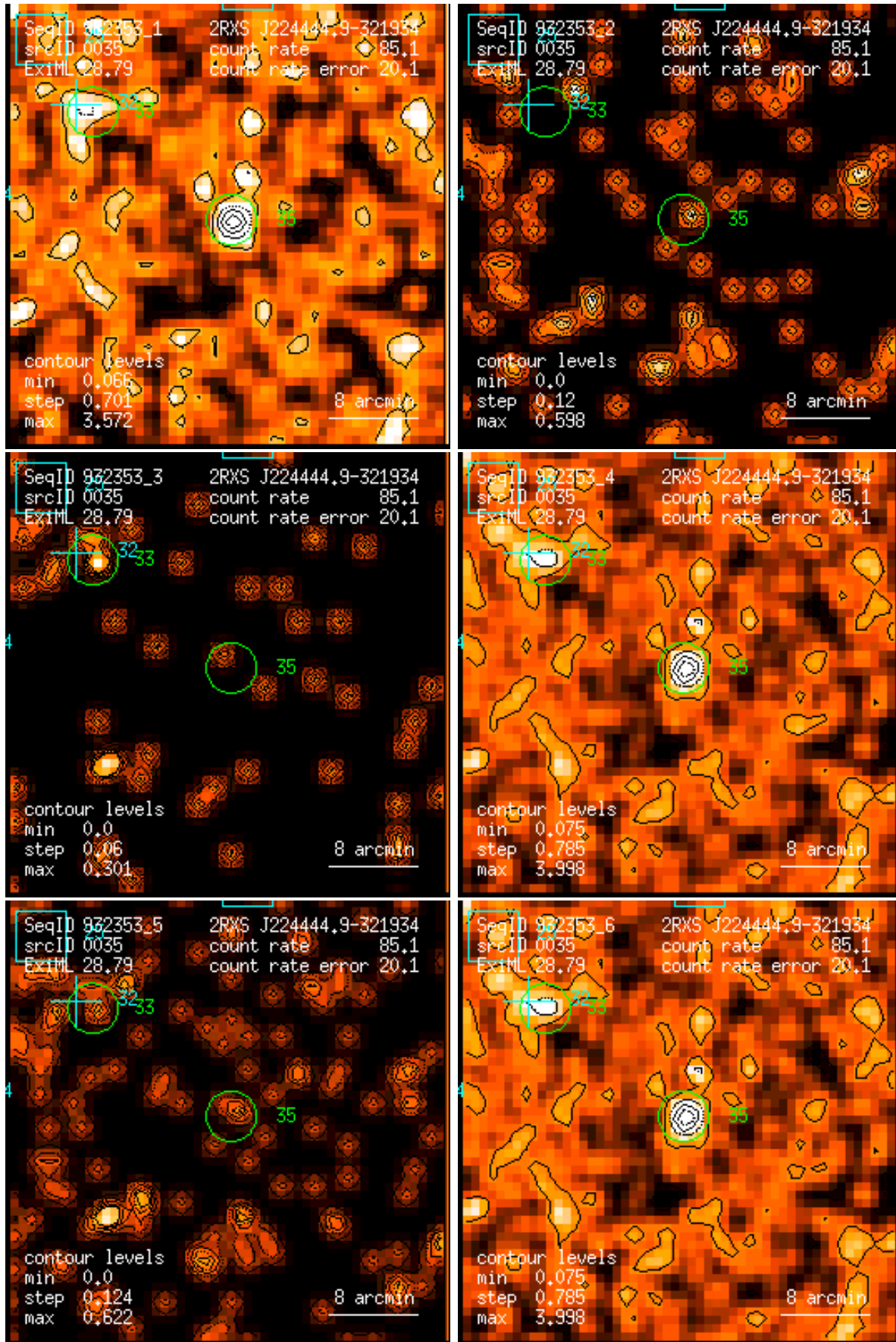
Figure 35: RASS 932353: detection 0035: band rate images, Gaussian filter: (1) PSPC channels 11 – 41, (2) 52 – 90, (3) 91 – 201, (4) 11 – 235, (5) 52 – 201, (6) 11 – 201. Broad band rates in counts/ks. Band rate contour levels in counts/ks/arcmin 2 .
