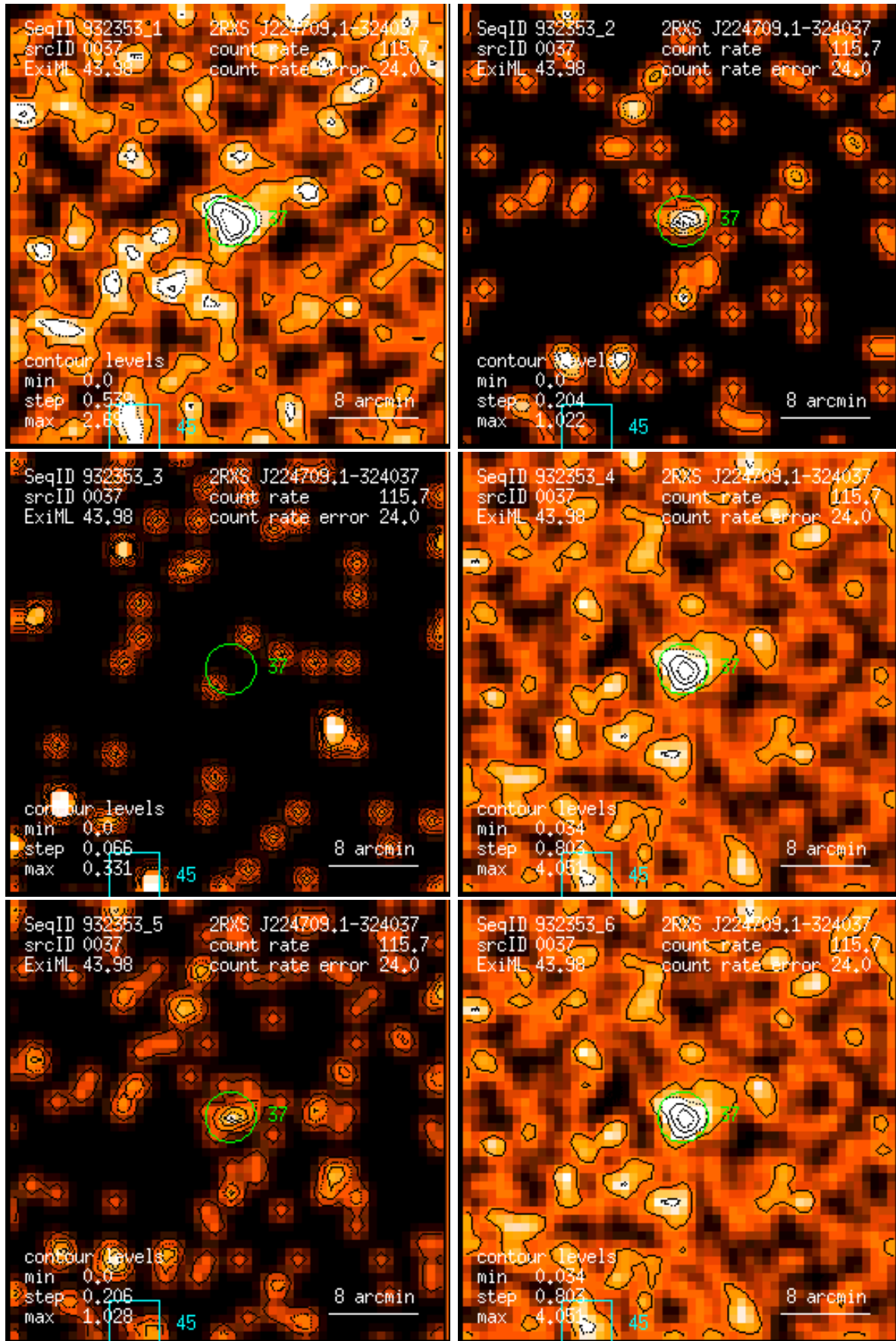
Figure 37: RASS 932353: detection 0037: band rate images, Gaussian filter: (1) PSPC channels 11 – 41, (2) 52 – 90, (3) 91 – 201, (4) 11 – 235, (5) 52 – 201, (6) 11 – 201. Broad band rates in counts/ks. Band rate contour levels in counts/ks/arcmin 2 .
