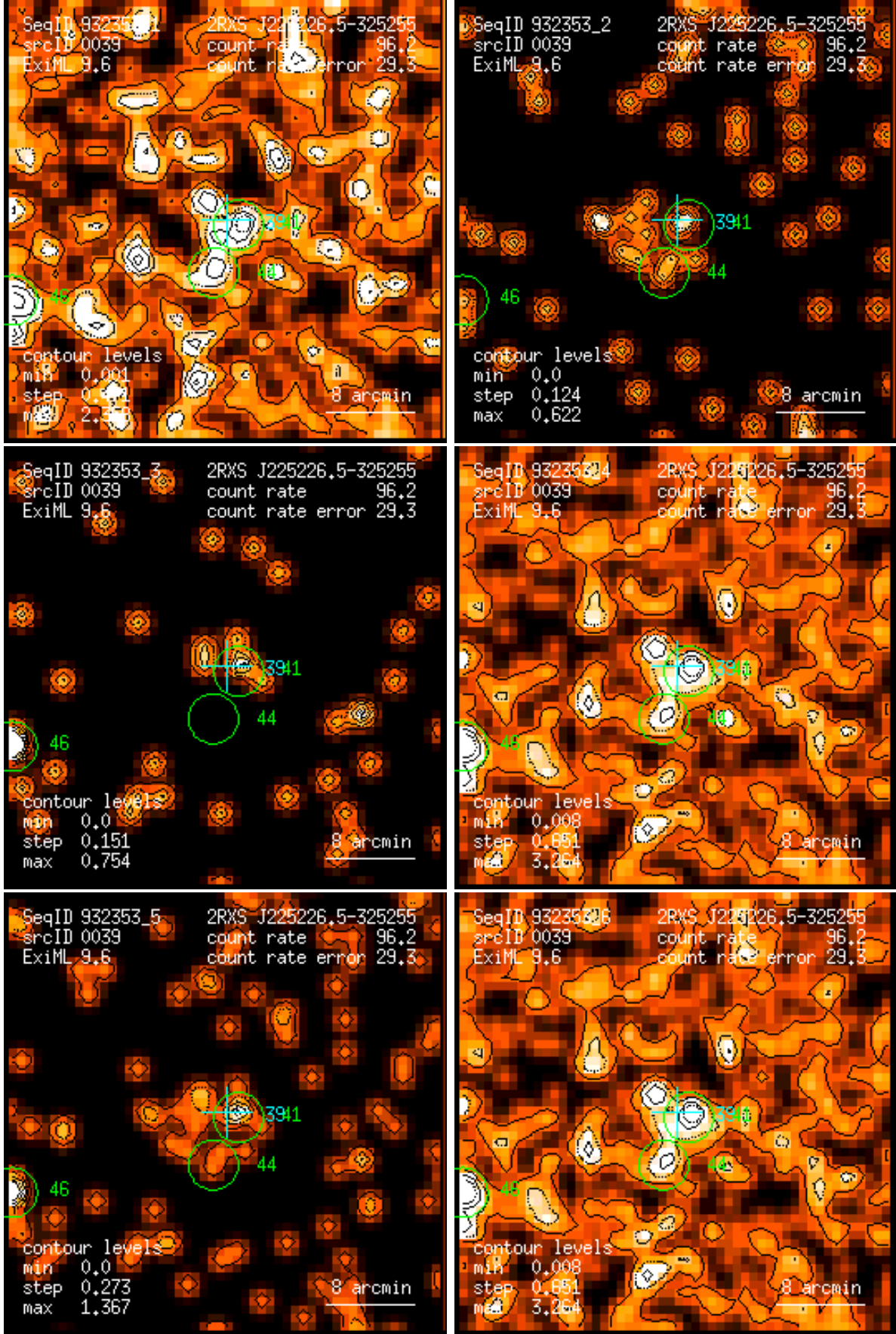
Figure 39: RASS 932353: detection 0039: band rate images, Gaussian filter: (1) PSPC channels 11 – 41, (2) 52 – 90, (3) 91 – 201, (4) 11 – 235, (5) 52 – 201, (6) 11 – 201. Broad band rates in counts/ks. Band rate contour levels in counts/ks/arcmin 2 .
