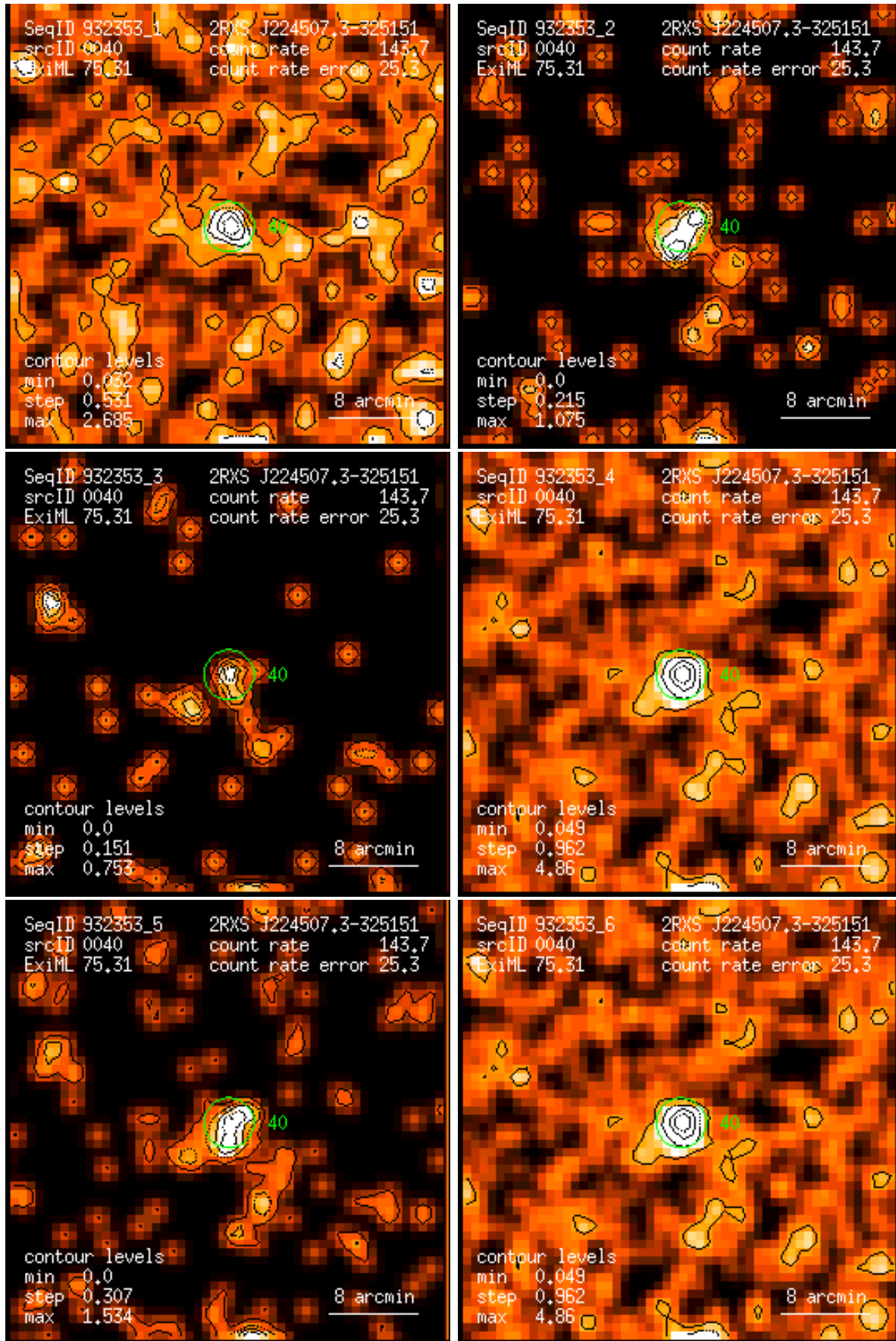
Figure 40: RASS 932353: detection 0040: band rate images, Gaussian filter: (1) PSPC channels 11 – 41, (2) 52 – 90, (3) 91 – 201, (4) 11 – 235, (5) 52 – 201, (6) 11 – 201. Broad band rates in counts/ks. Band rate contour levels in counts/ks/arcmin 2 .
