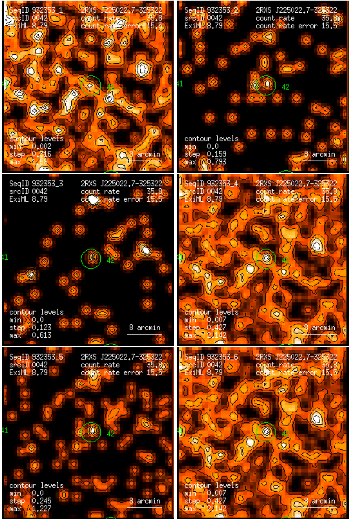
Figure 42: RASS 932353: detection 0042: band rate images, Gaussian filter: (1) PSPC channels 11 – 41, (2) 52 – 90, (3) 91 – 201, (4) 11 – 235, (5) 52 – 201, (6) 11 – 201. Broad band rates in counts/ks. Band rate contour levels in counts/ks/arcmin 2 .
