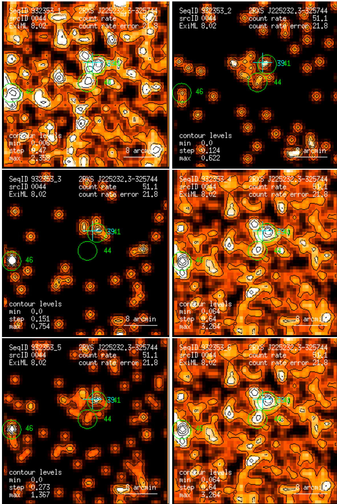
Figure 44: RASS 932353: detection 0044: band rate images, Gaussian filter: (1) PSPC channels 11 – 41, (2) 52 – 90, (3) 91 – 201, (4) 11 – 235, (5) 52 – 201, (6) 11 – 201. Broad band rates in counts/ks. Band rate contour levels in counts/ks/arcmin 2 .
