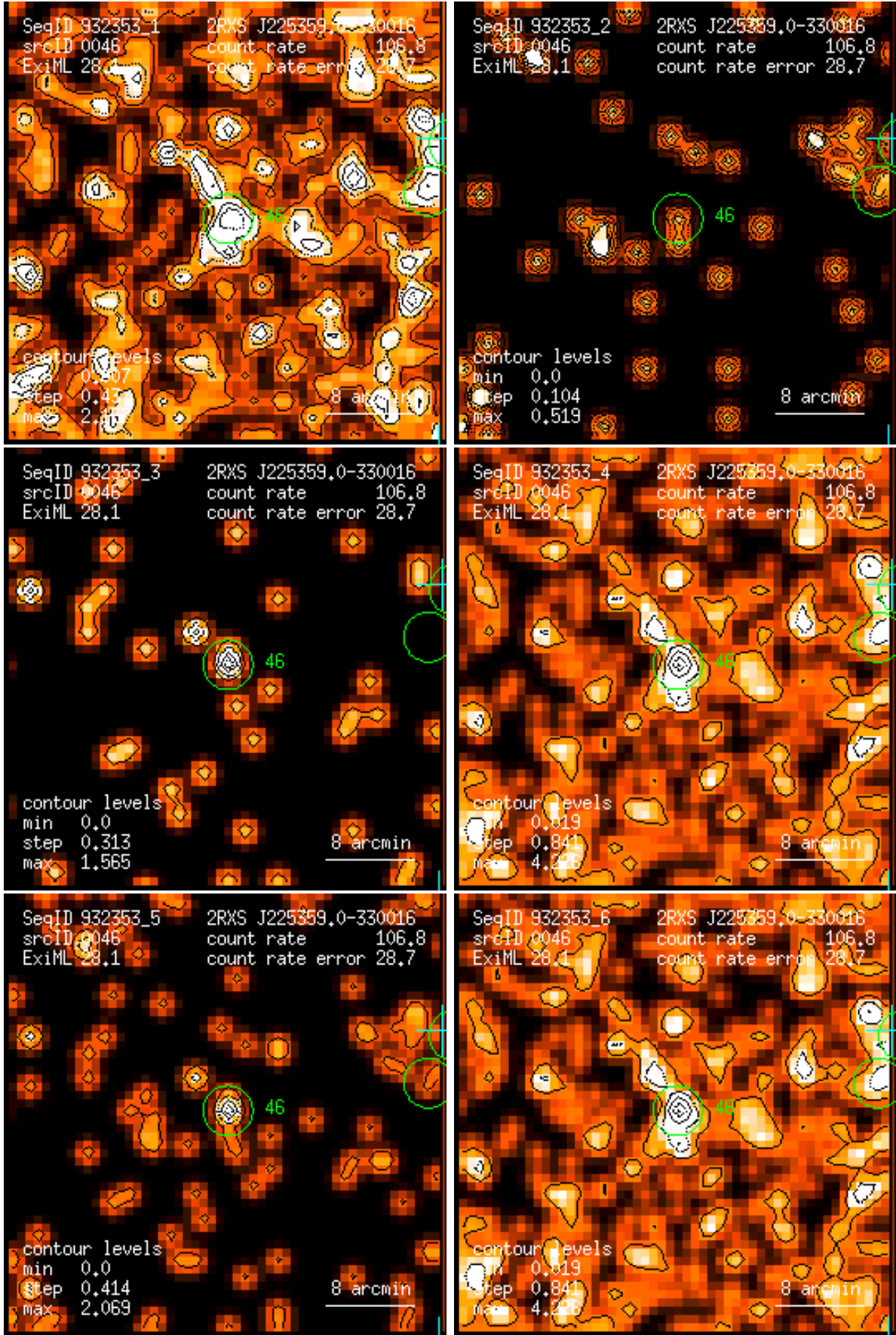
Figure 46: RASS 932353: detection 0046: band rate images, Gaussian filter: (1) PSPC channels 11 – 41, (2) 52 – 90, (3) 91 – 201, (4) 11 – 235, (5) 52 – 201, (6) 11 – 201. Broad band rates in counts/ks. Band rate contour levels in counts/ks/arcmin 2 .
