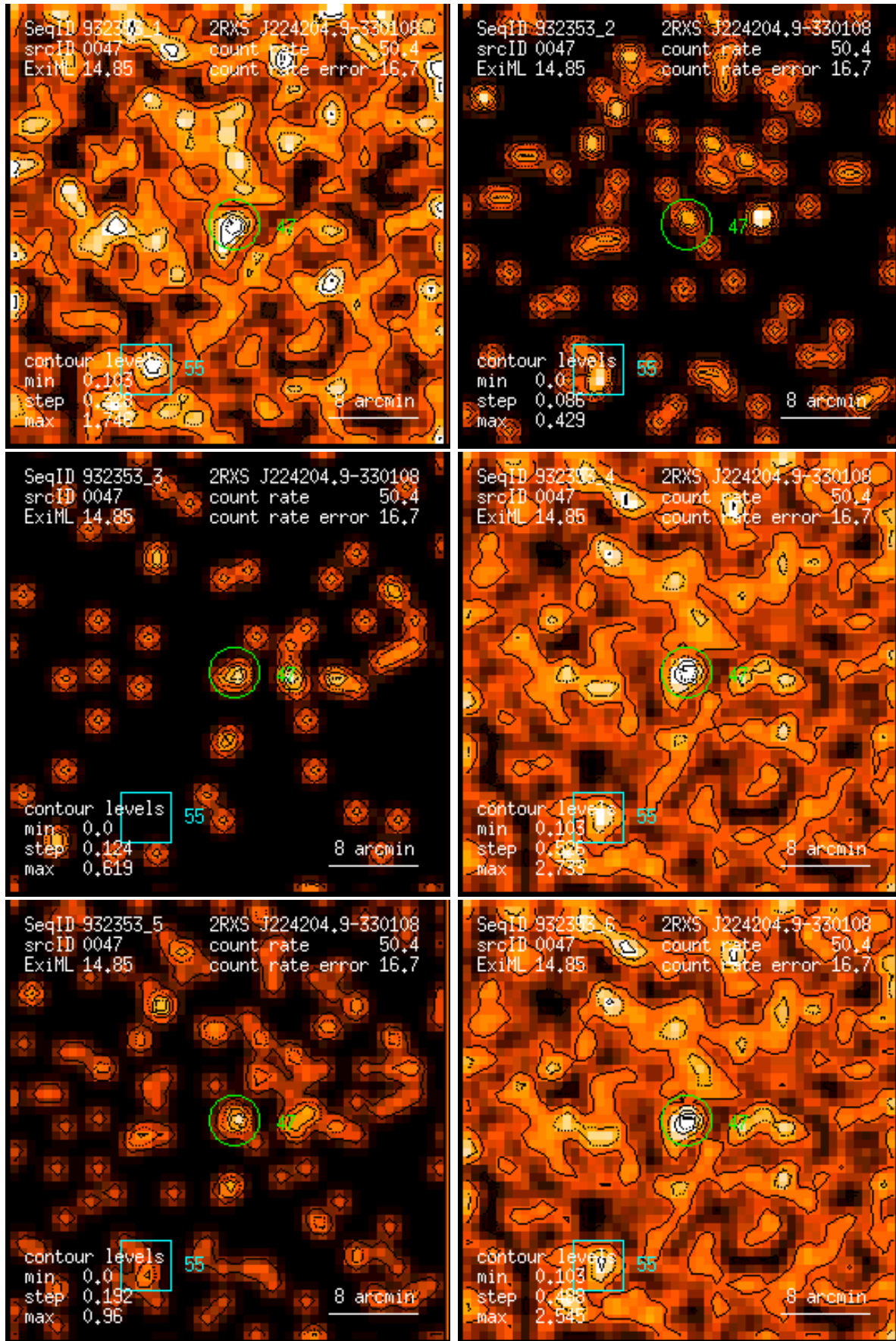
Figure 47: RASS 932353: detection 0047: band rate images, Gaussian filter: (1) PSPC channels 11 – 41, (2) 52 – 90, (3) 91 – 201, (4) 11 – 235, (5) 52 – 201, (6) 11 – 201. Broad band rates in counts/ks. Band rate contour levels in counts/ks/arcmin 2 .
