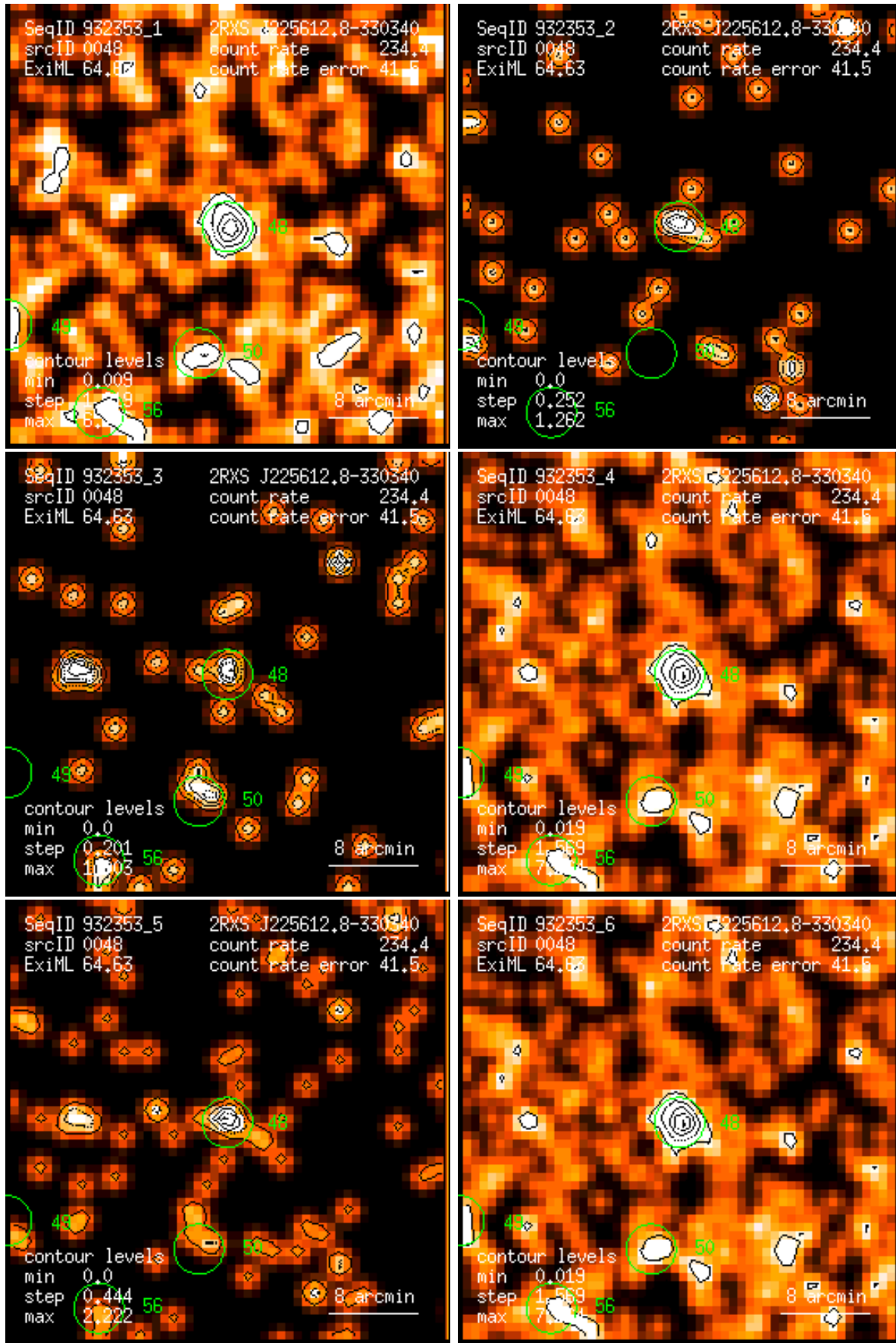
Figure 48: RASS 932353: detection 0048: band rate images, Gaussian filter: (1) PSPC channels 11 – 41, (2) 52 – 90, (3) 91 – 201, (4) 11 – 235, (5) 52 – 201, (6) 11 – 201. Broad band rates in counts/ks. Band rate contour levels in counts/ks/arcmin 2 .
