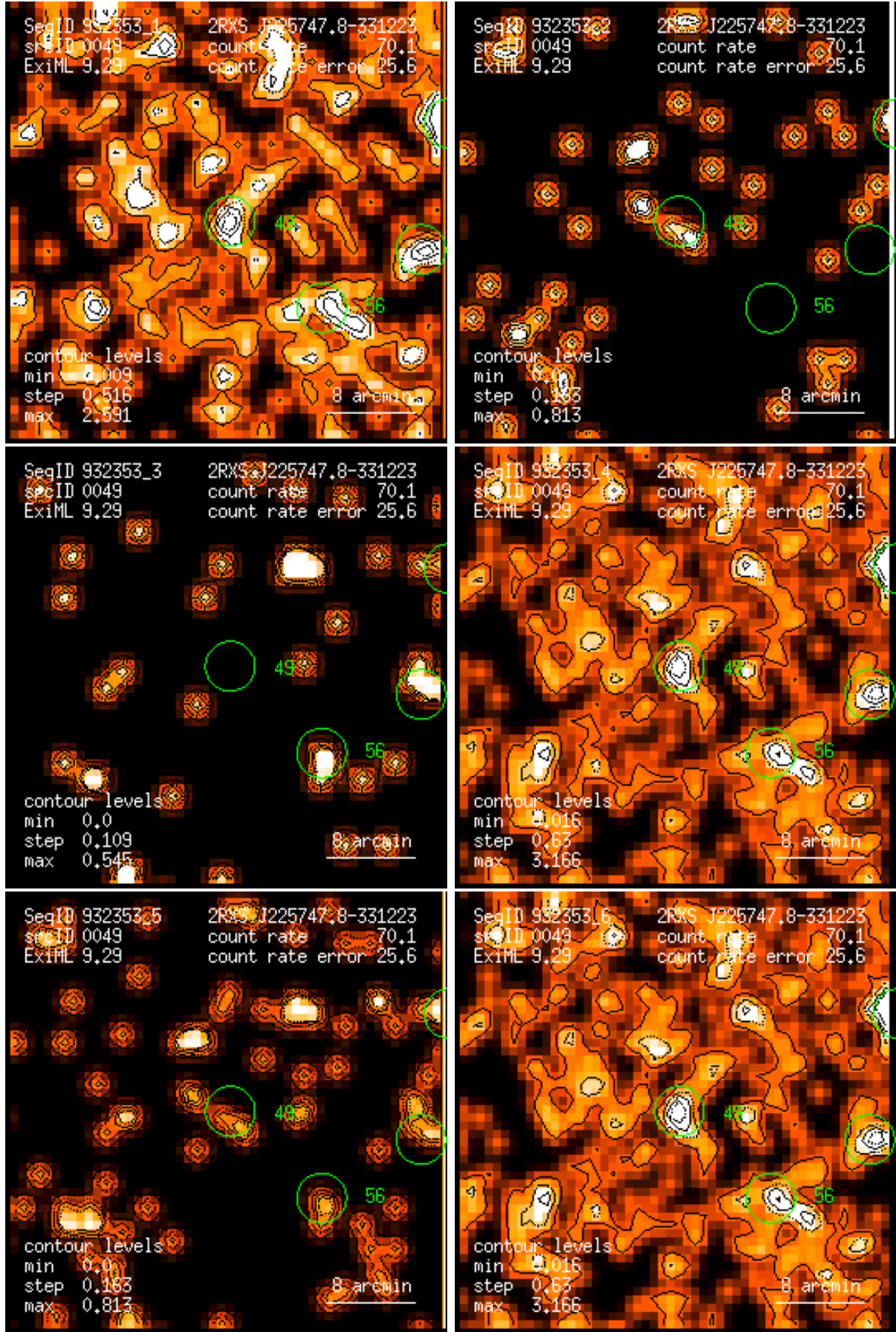
Figure 49: RASS 932353: detection 0049: band rate images, Gaussian filter: (1) PSPC channels 11 – 41, (2) 52 – 90, (3) 91 – 201, (4) 11 – 235, (5) 52 – 201, (6) 11 – 201. Broad band rates in counts/ks. Band rate contour levels in counts/ks/arcmin 2 .
