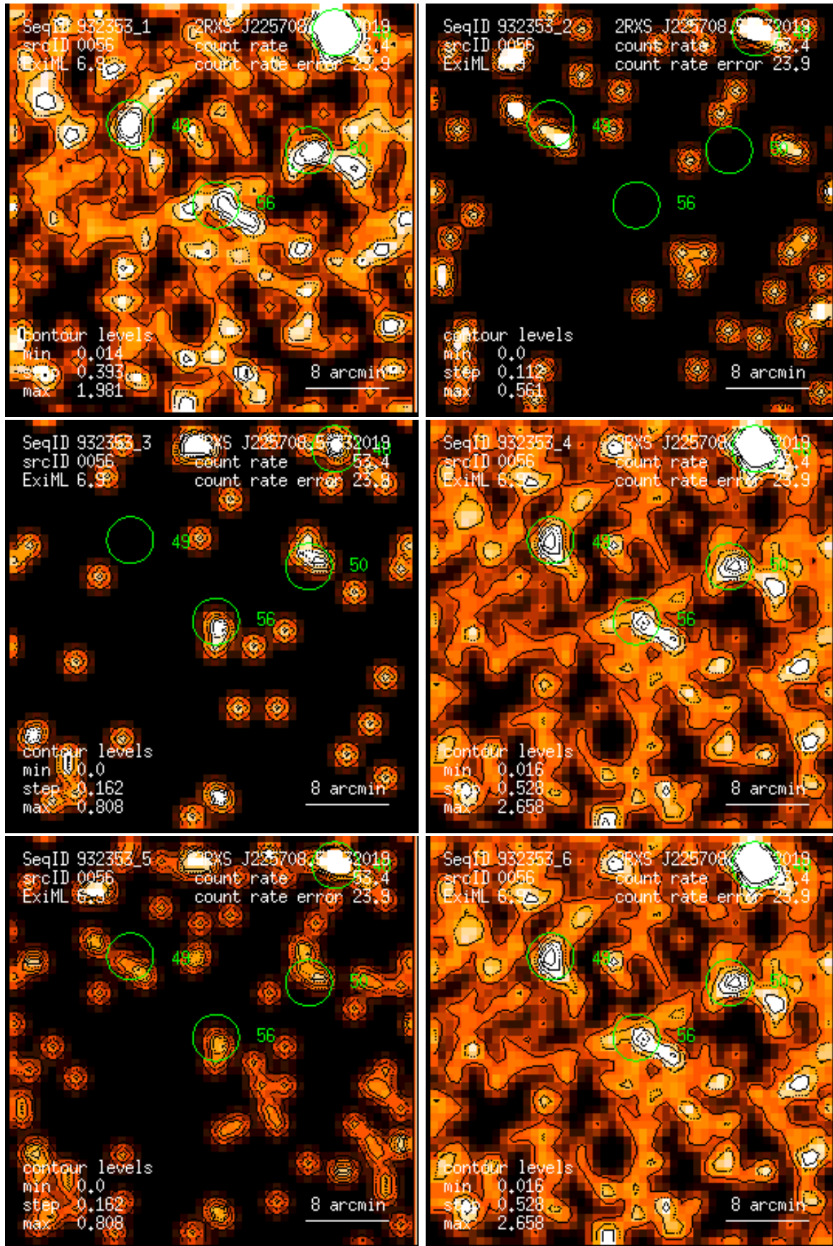
Figure 56: RASS 932353: detection 0056: band rate images, Gaussian filter: (1) PSPC channels 11 – 41, (2) 52 – 90, (3) 91 – 201, (4) 11 – 235, (5) 52 – 201, (6) 11 – 201. Broad band rates in counts/ks. Band rate contour levels in counts/ks/arcmin 2 .
