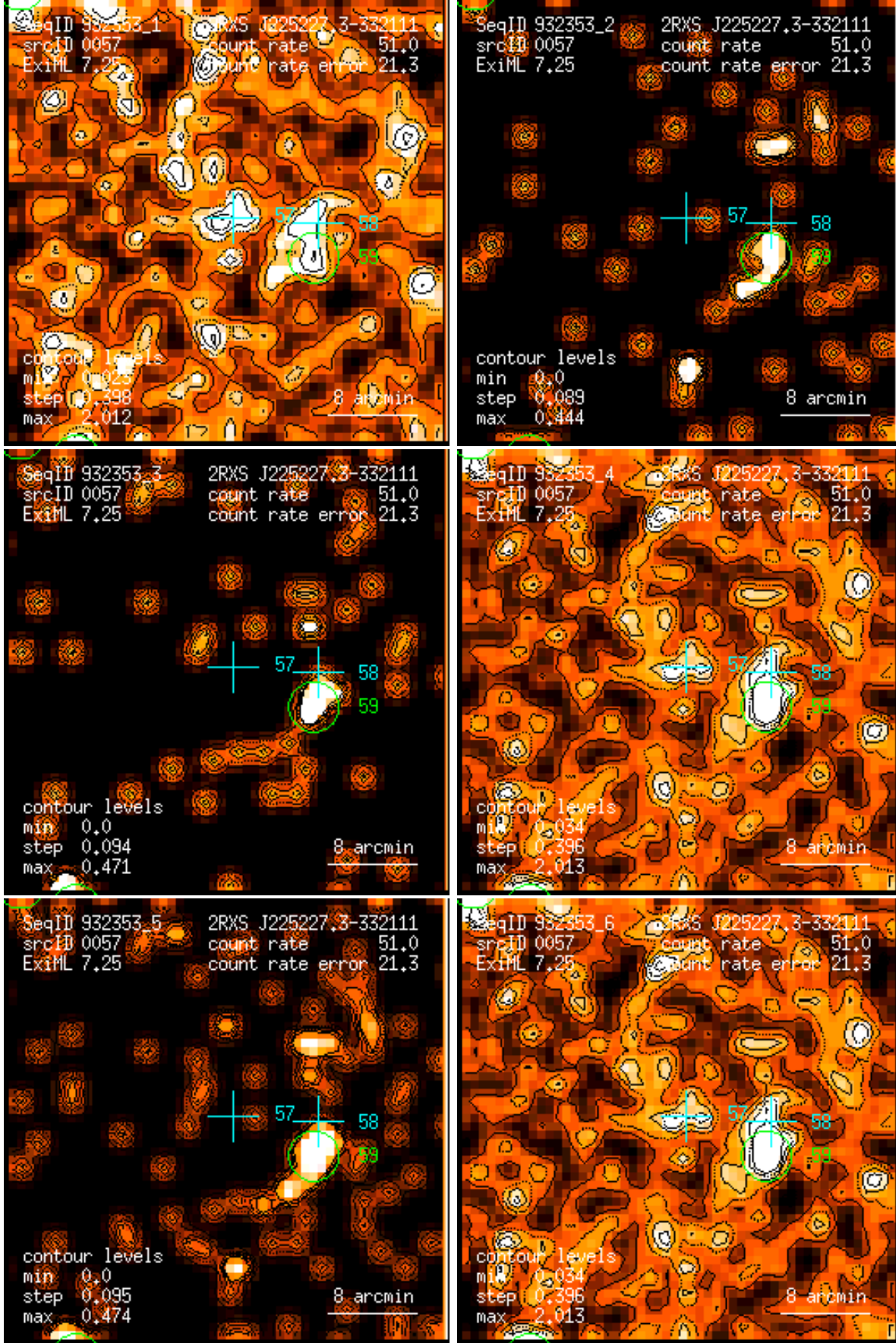
Figure 57: RASS 932353: detection 0057: band rate images, Gaussian filter: (1) PSPC channels 11 – 41, (2) 52 – 90, (3) 91 – 201, (4) 11 – 235, (5) 52 – 201, (6) 11 – 201. Broad band rates in counts/ks. Band rate contour levels in counts/ks/arcmin 2 .
