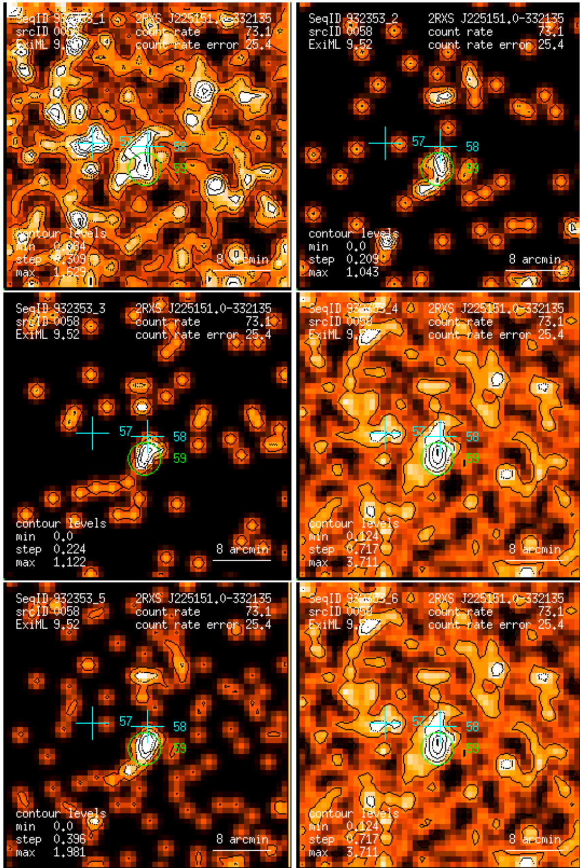
Figure 58: RASS 932353: detection 0058: band rate images, Gaussian filter: (1) PSPC channels 11 – 41, (2) 52 – 90, (3) 91 – 201, (4) 11 – 235, (5) 52 – 201, (6) 11 – 201. Broad band rates in counts/ks. Band rate contour levels in counts/ks/arcmin 2 .
