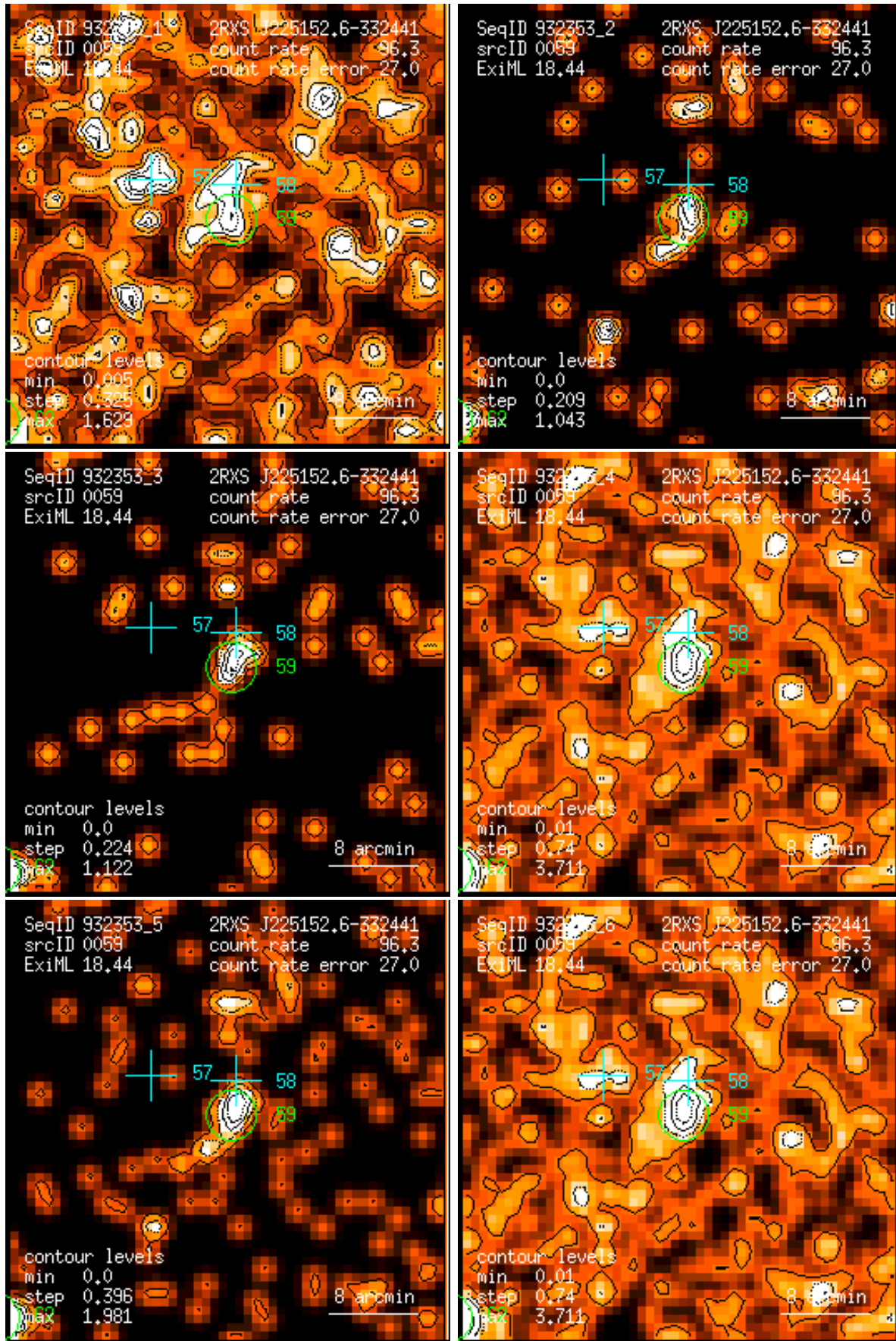
Figure 59: RASS 932353: detection 0059: band rate images, Gaussian filter: (1) PSPC channels 11 – 41, (2) 52 – 90, (3) 91 – 201, (4) 11 – 235, (5) 52 – 201, (6) 11 – 201. Broad band rates in counts/ks. Band rate contour levels in counts/ks/arcmin 2 .
