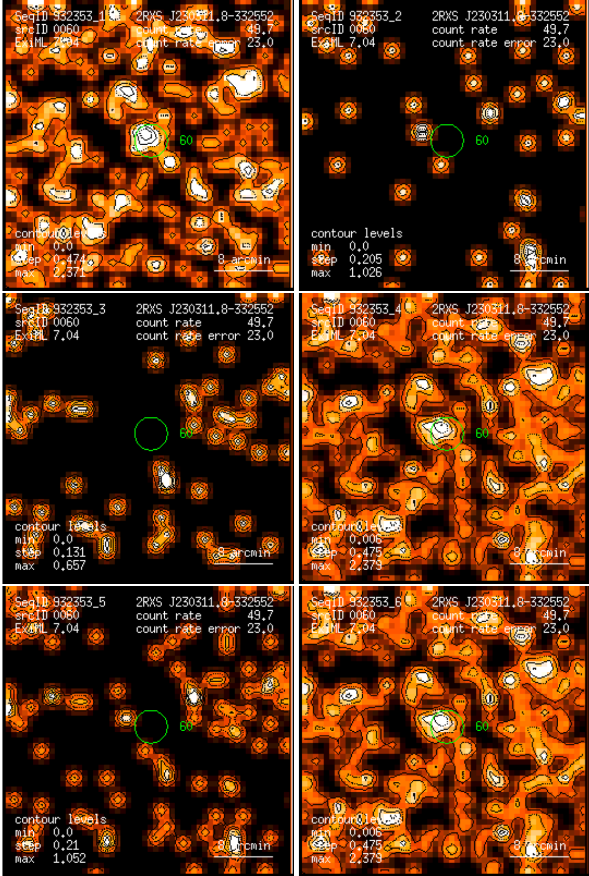
Figure 60: RASS 932353: detection 0060: band rate images, Gaussian filter: (1) PSPC channels 11 – 41, (2) 52 – 90, (3) 91 – 201, (4) 11 – 235, (5) 52 – 201, (6) 11 – 201. Broad band rates in counts/ks. Band rate contour levels in counts/ks/arcmin 2 .
