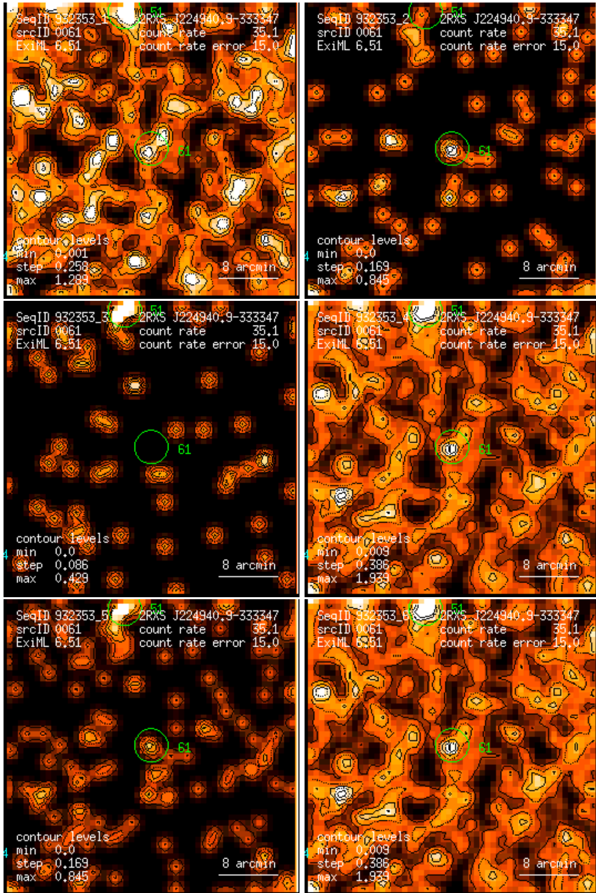
Figure 61: RASS 932353: detection 0061: band rate images, Gaussian filter: (1) PSPC channels 11 – 41, (2) 52 – 90, (3) 91 – 201, (4) 11 – 235, (5) 52 – 201, (6) 11 – 201. Broad band rates in counts/ks. Band rate contour levels in counts/ks/arcmin 2 .
