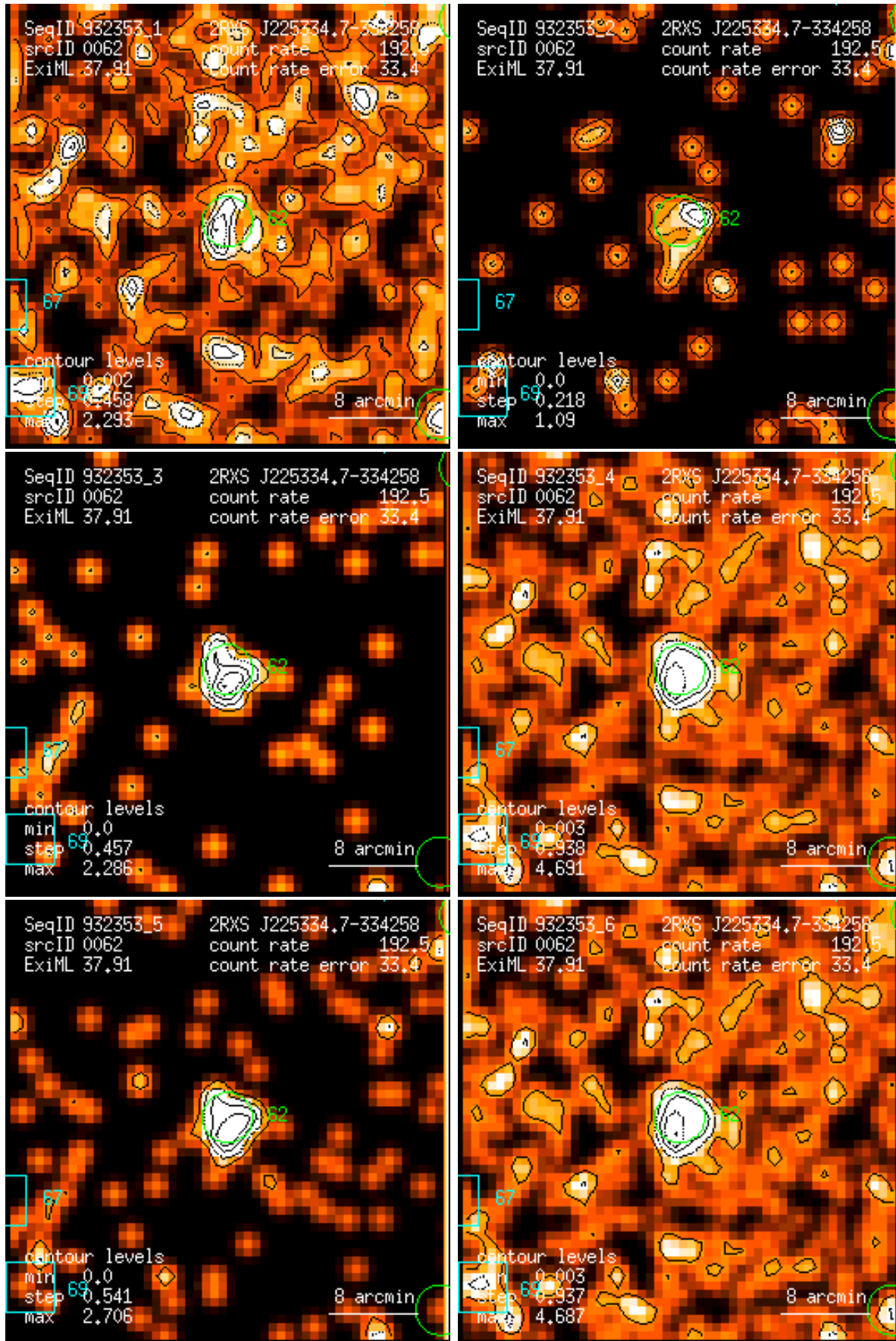
Figure 62: RASS 932353: detection 0062: band rate images, Gaussian filter: (1) PSPC channels 11 – 41, (2) 52 – 90, (3) 91 – 201, (4) 11 – 235, (5) 52 – 201, (6) 11 – 201. Broad band rates in counts/ks. Band rate contour levels in counts/ks/arcmin 2 .
