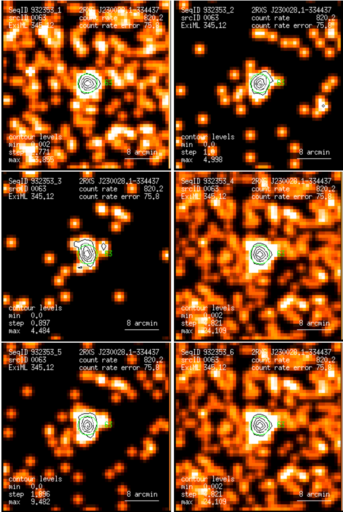
Figure 63: RASS 932353: detection 0063: band rate images, Gaussian filter: (1) PSPC channels 11 – 41, (2) 52 – 90, (3) 91 – 201, (4) 11 – 235, (5) 52 – 201, (6) 11 – 201. Broad band rates in counts/ks. Band rate contour levels in counts/ks/arcmin 2 .
