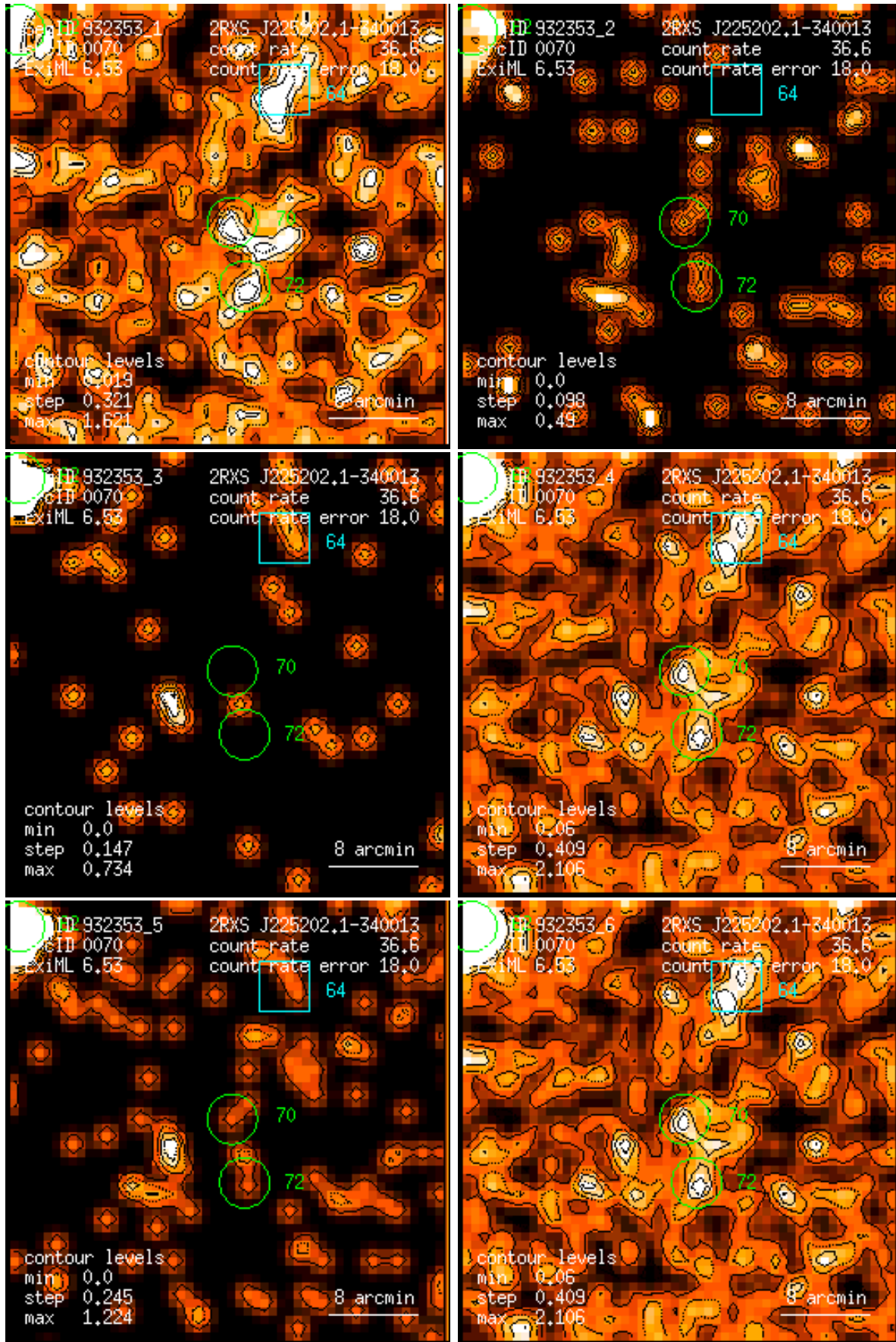
Figure 70: RASS 932353: detection 0070: band rate images, Gaussian filter: (1) PSPC channels 11 – 41, (2) 52 – 90, (3) 91 – 201, (4) 11 – 235, (5) 52 – 201, (6) 11 – 201. Broad band rates in counts/ks. Band rate contour levels in counts/ks/arcmin 2 .
