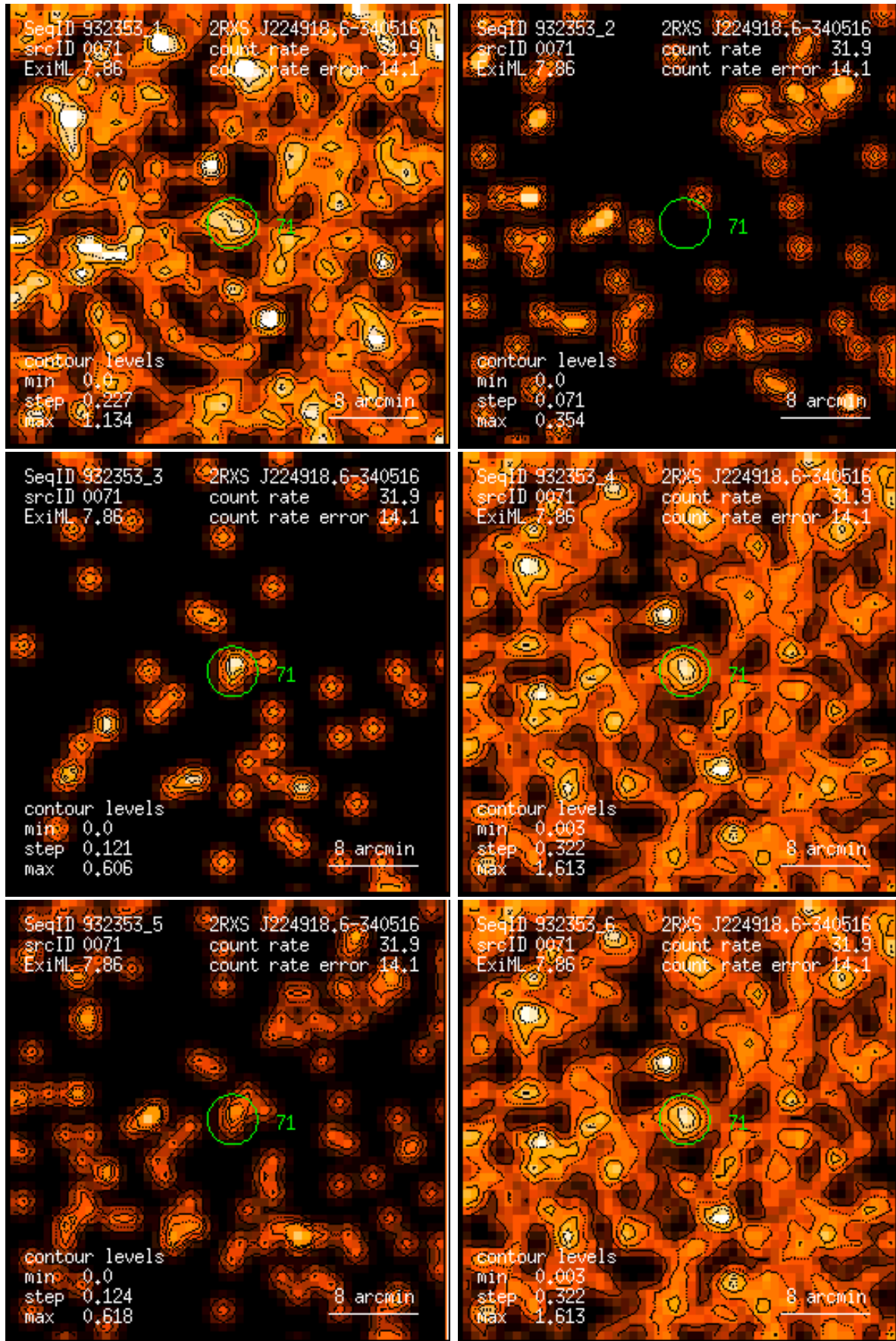
Figure 71: RASS 932353: detection 0071: band rate images, Gaussian filter: (1) PSPC channels 11 – 41, (2) 52 – 90, (3) 91 – 201, (4) 11 – 235, (5) 52 – 201, (6) 11 – 201. Broad band rates in counts/ks. Band rate contour levels in counts/ks/arcmin 2 .
