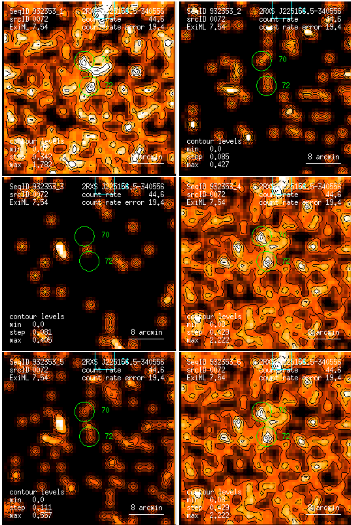
Figure 72: RASS 932353: detection 0072: band rate images, Gaussian filter: (1) PSPC channels 11 – 41, (2) 52 – 90, (3) 91 – 201, (4) 11 – 235, (5) 52 – 201, (6) 11 – 201. Broad band rates in counts/ks. Band rate contour levels in counts/ks/arcmin 2 .
