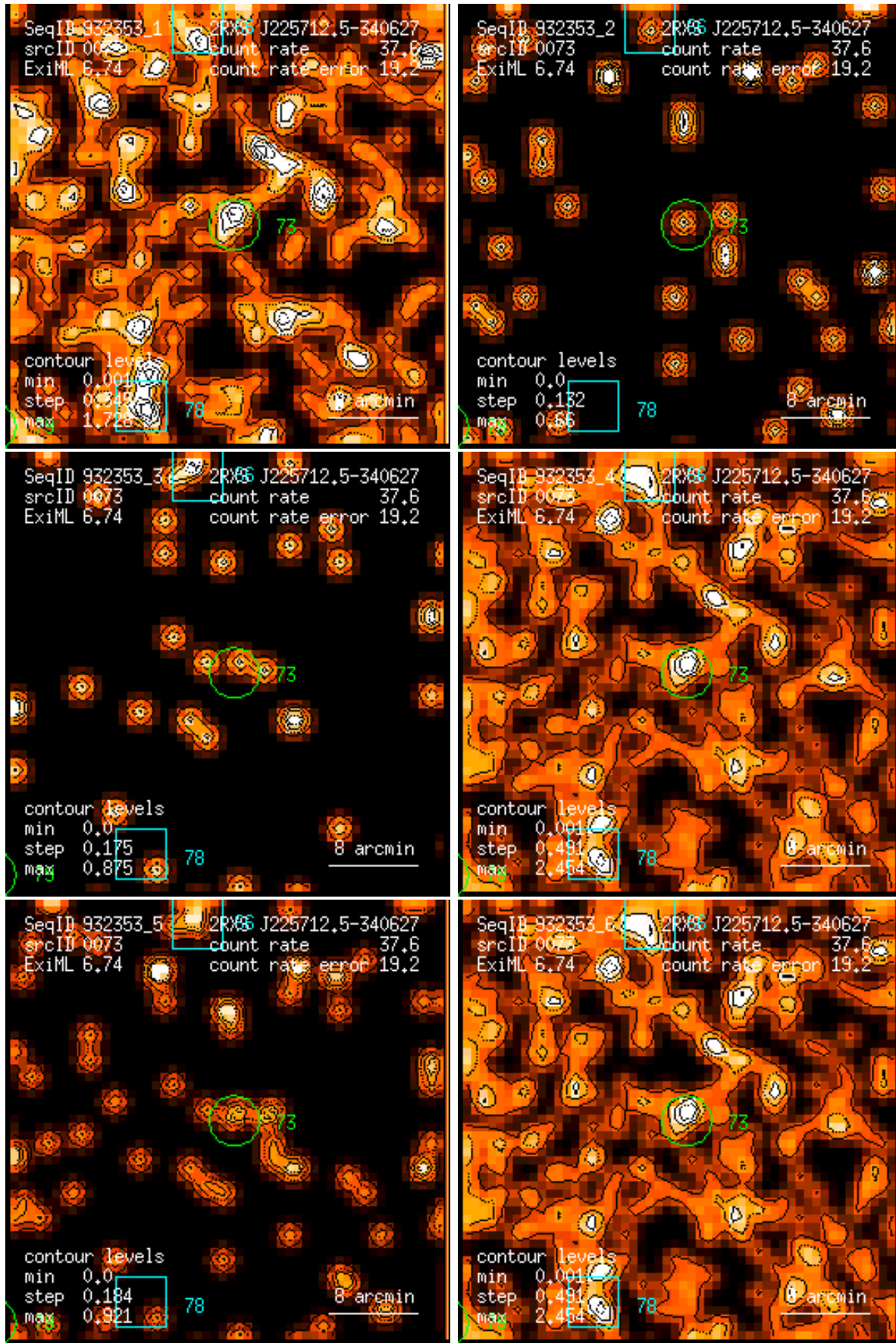
Figure 73: RASS 932353: detection 0073: band rate images, Gaussian filter: (1) PSPC channels 11 – 41, (2) 52 – 90, (3) 91 – 201, (4) 11 – 235, (5) 52 – 201, (6) 11 – 201. Broad band rates in counts/ks. Band rate contour levels in counts/ks/arcmin 2 .
