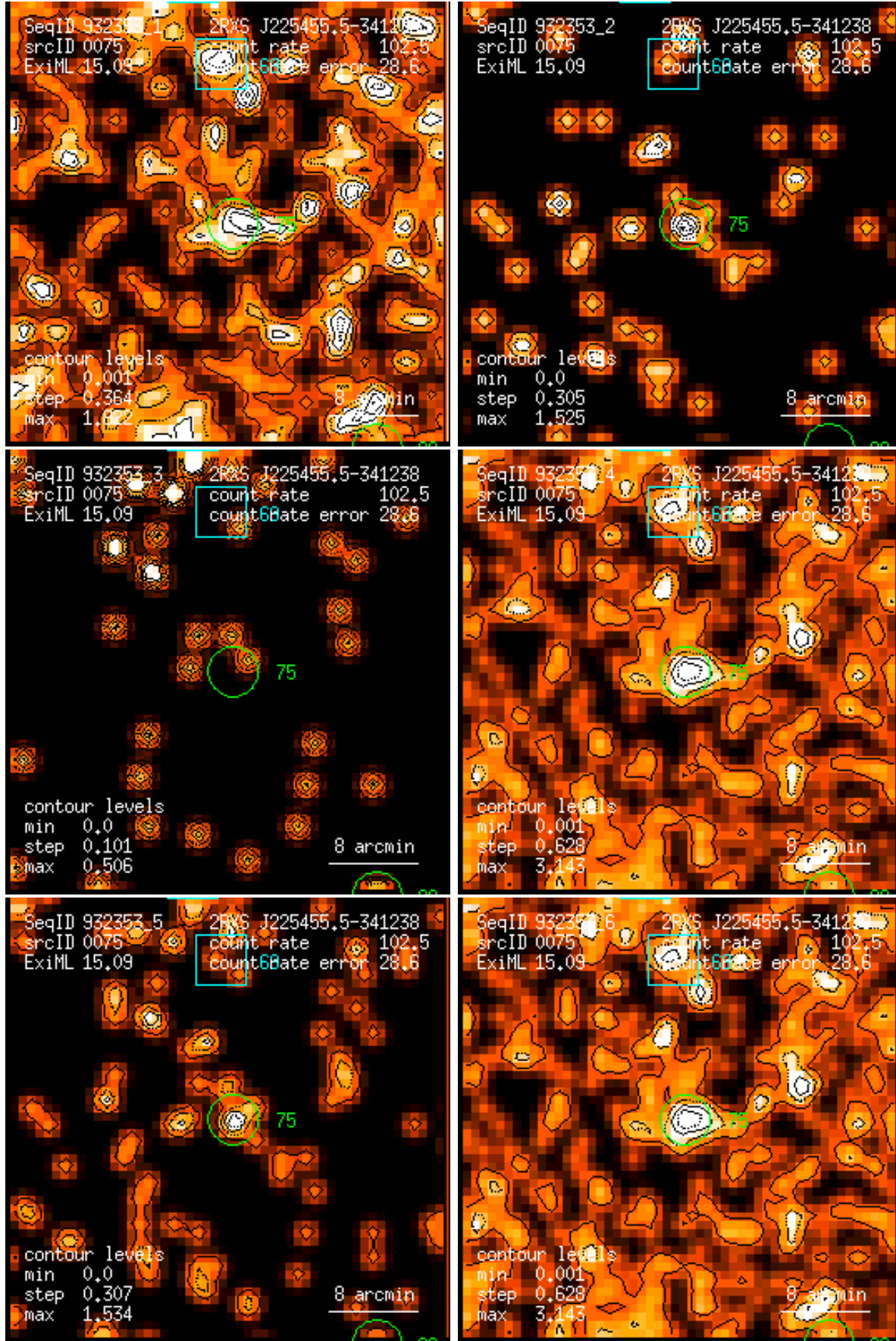
Figure 75: RASS 932353: detection 0075: band rate images, Gaussian filter: (1) PSPC channels 11 – 41, (2) 52 – 90, (3) 91 – 201, (4) 11 – 235, (5) 52 – 201, (6) 11 – 201. Broad band rates in counts/ks. Band rate contour levels in counts/ks/arcmin 2 .
