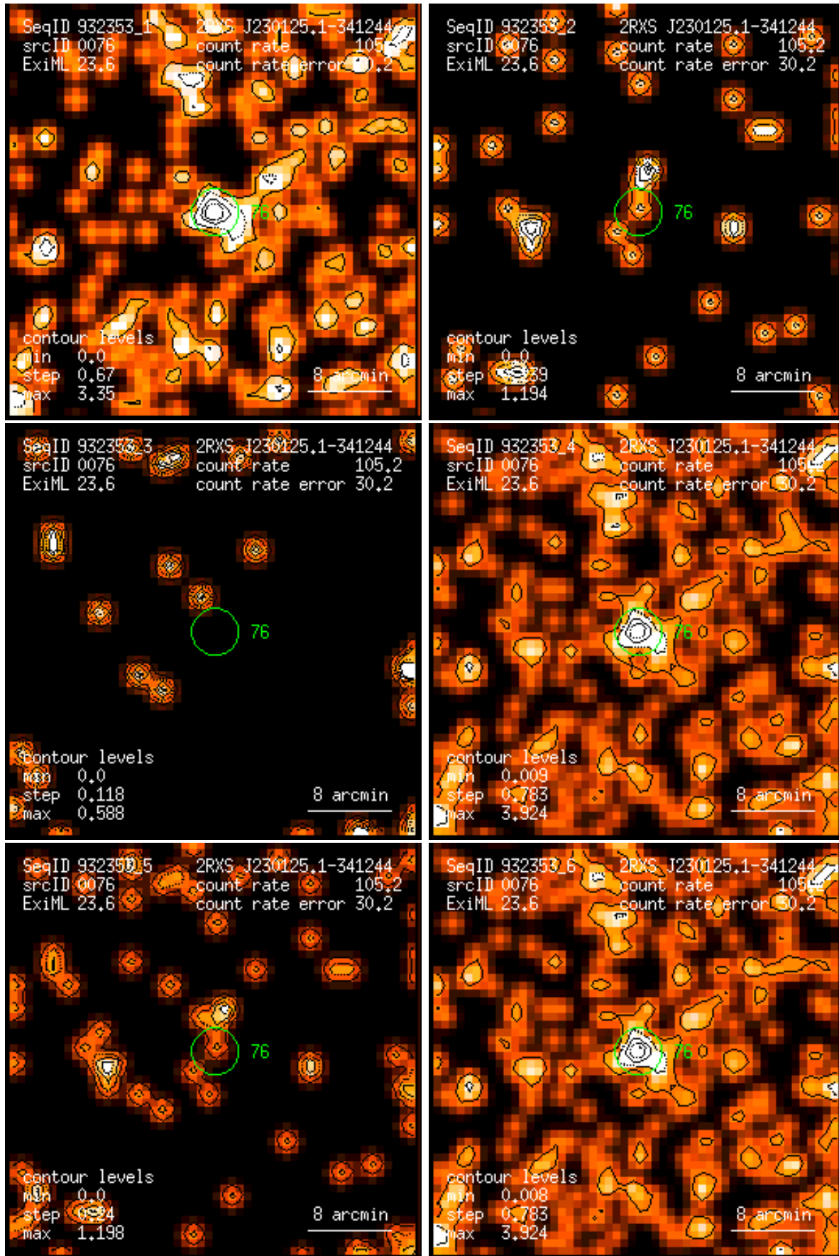
Figure 76: RASS 932353: detection 0076: band rate images, Gaussian filter: (1) PSPC channels 11 – 41, (2) 52 – 90, (3) 91 – 201, (4) 11 – 235, (5) 52 – 201, (6) 11 – 201. Broad band rates in counts/ks. Band rate contour levels in counts/ks/arcmin 2 .
