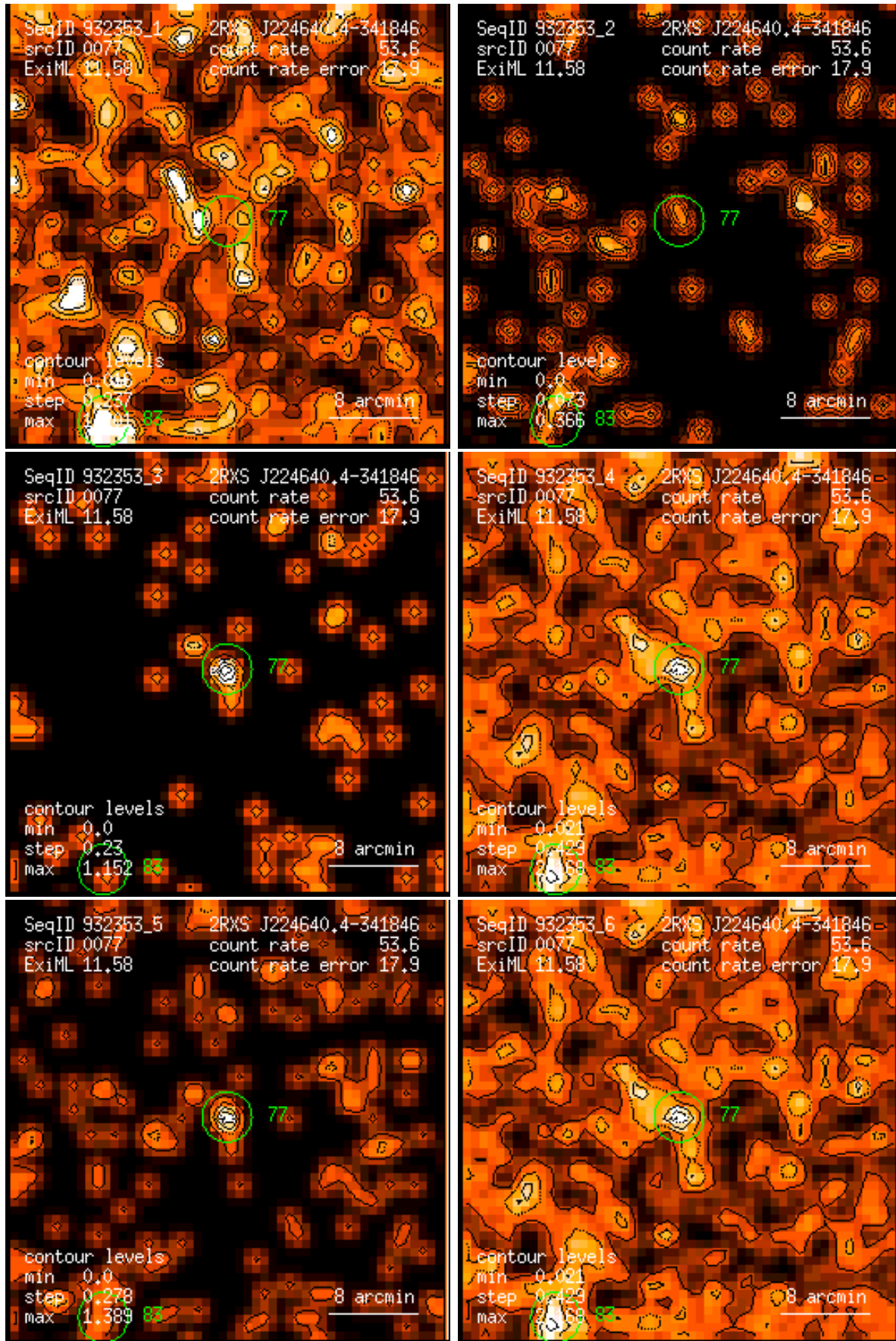
Figure 77: RASS 932353: detection 0077: band rate images, Gaussian filter: (1) PSPC channels 11 – 41, (2) 52 – 90, (3) 91 – 201, (4) 11 – 235, (5) 52 – 201, (6) 11 – 201. Broad band rates in counts/ks. Band rate contour levels in counts/ks/arcmin 2 .
