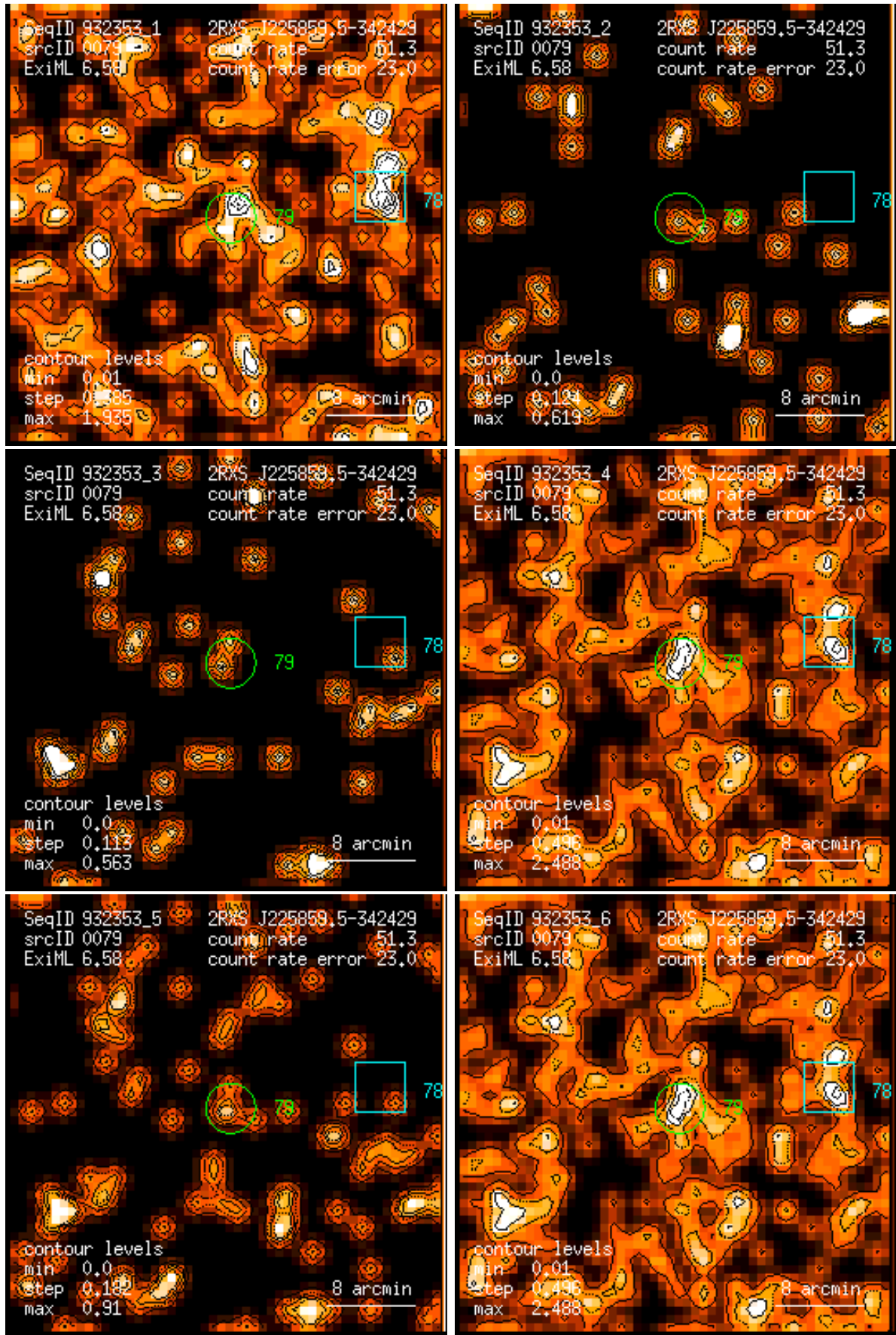
Figure 79: RASS 932353: detection 0079: band rate images, Gaussian filter: (1) PSPC channels 11 – 41, (2) 52 – 90, (3) 91 – 201, (4) 11 – 235, (5) 52 – 201, (6) 11 – 201. Broad band rates in counts/ks. Band rate contour levels in counts/ks/arcmin 2 .
