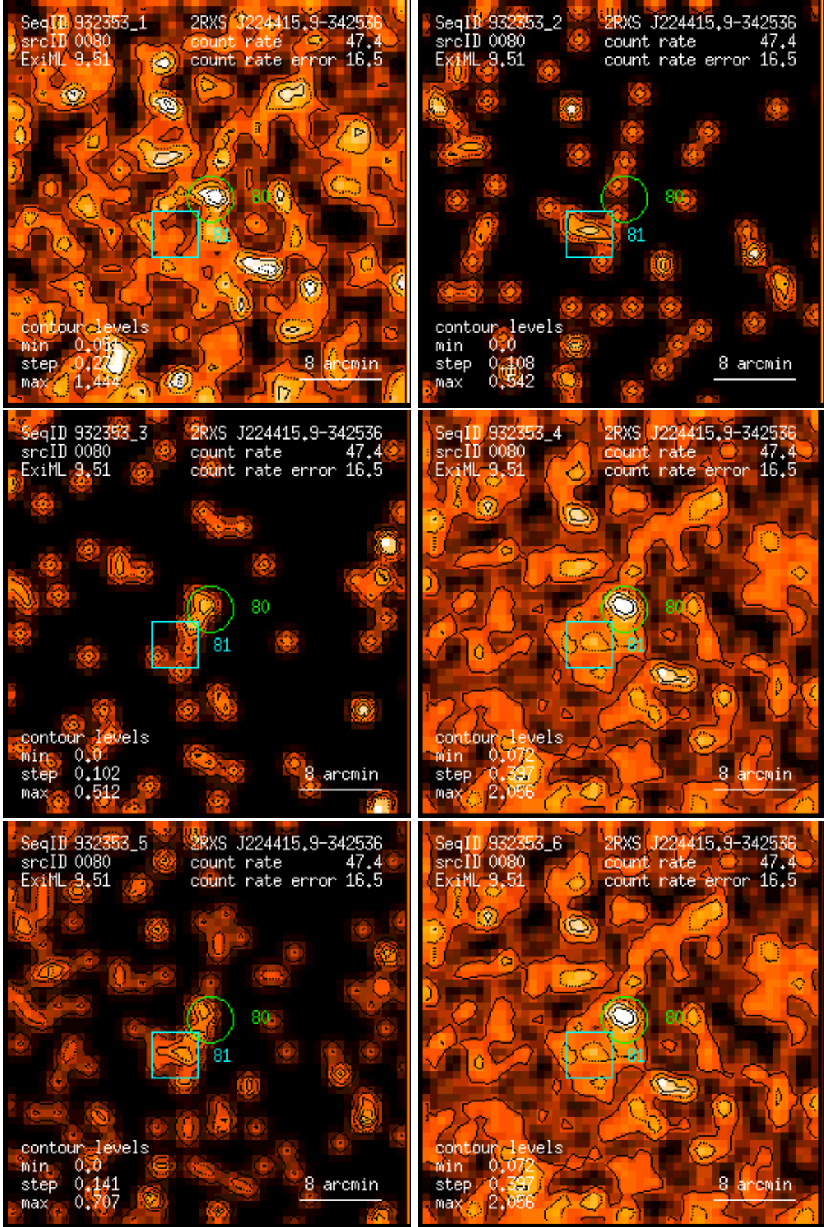
Figure 80: RASS 932353: detection 0080: band rate images, Gaussian filter: (1) PSPC channels 11 – 41, (2) 52 – 90, (3) 91 – 201, (4) 11 – 235, (5) 52 – 201, (6) 11 – 201. Broad band rates in counts/ks. Band rate contour levels in counts/ks/arcmin 2 .
