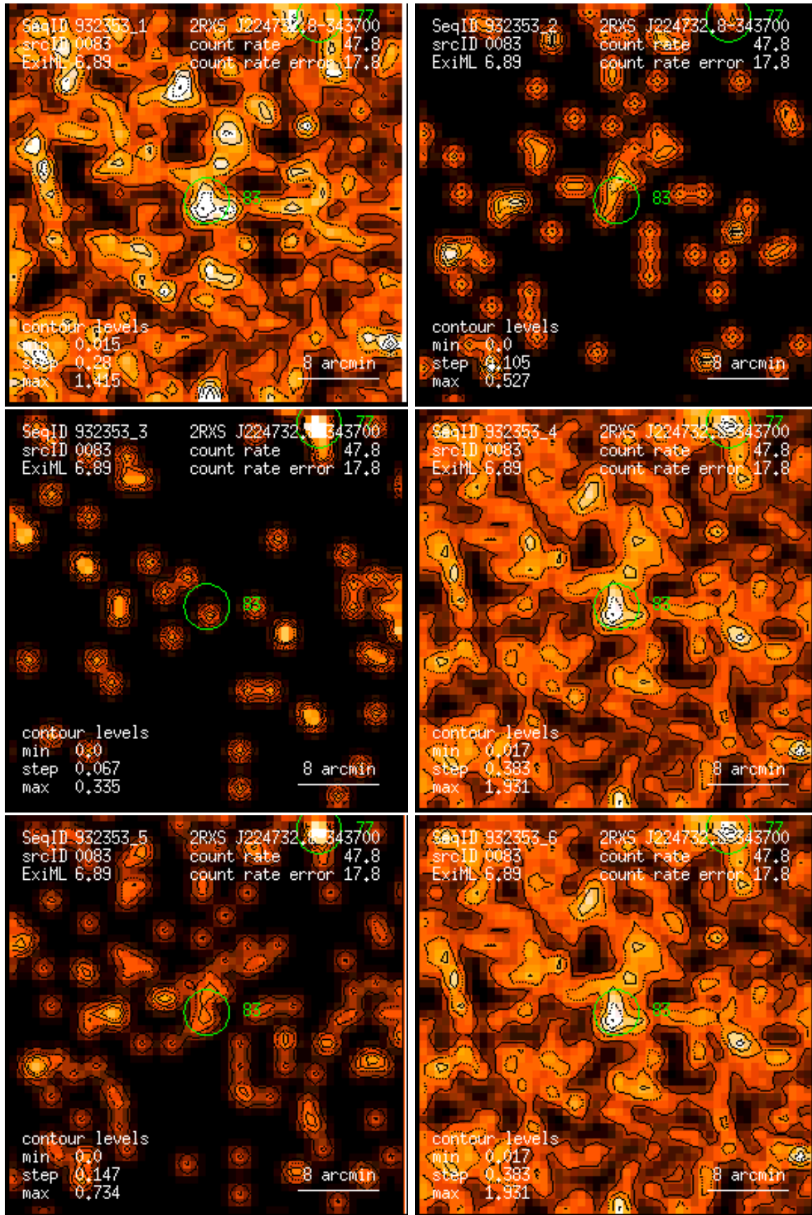
Figure 83: RASS 932353: detection 0083: band rate images, Gaussian filter: (1) PSPC channels 11 – 41, (2) 52 – 90, (3) 91 – 201, (4) 11 – 235, (5) 52 – 201, (6) 11 – 201. Broad band rates in counts/ks. Band rate contour levels in counts/ks/arcmin 2 .
