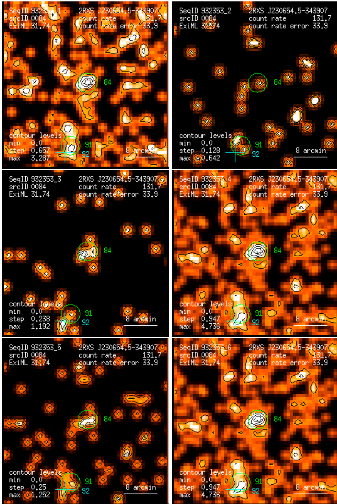
Figure 84: RASS 932353: detection 0084: band rate images, Gaussian filter: (1) PSPC channels 11 – 41, (2) 52 – 90, (3) 91 – 201, (4) 11 – 235, (5) 52 – 201, (6) 11 – 201. Broad band rates in counts/ks. Band rate contour levels in counts/ks/arcmin 2 .
