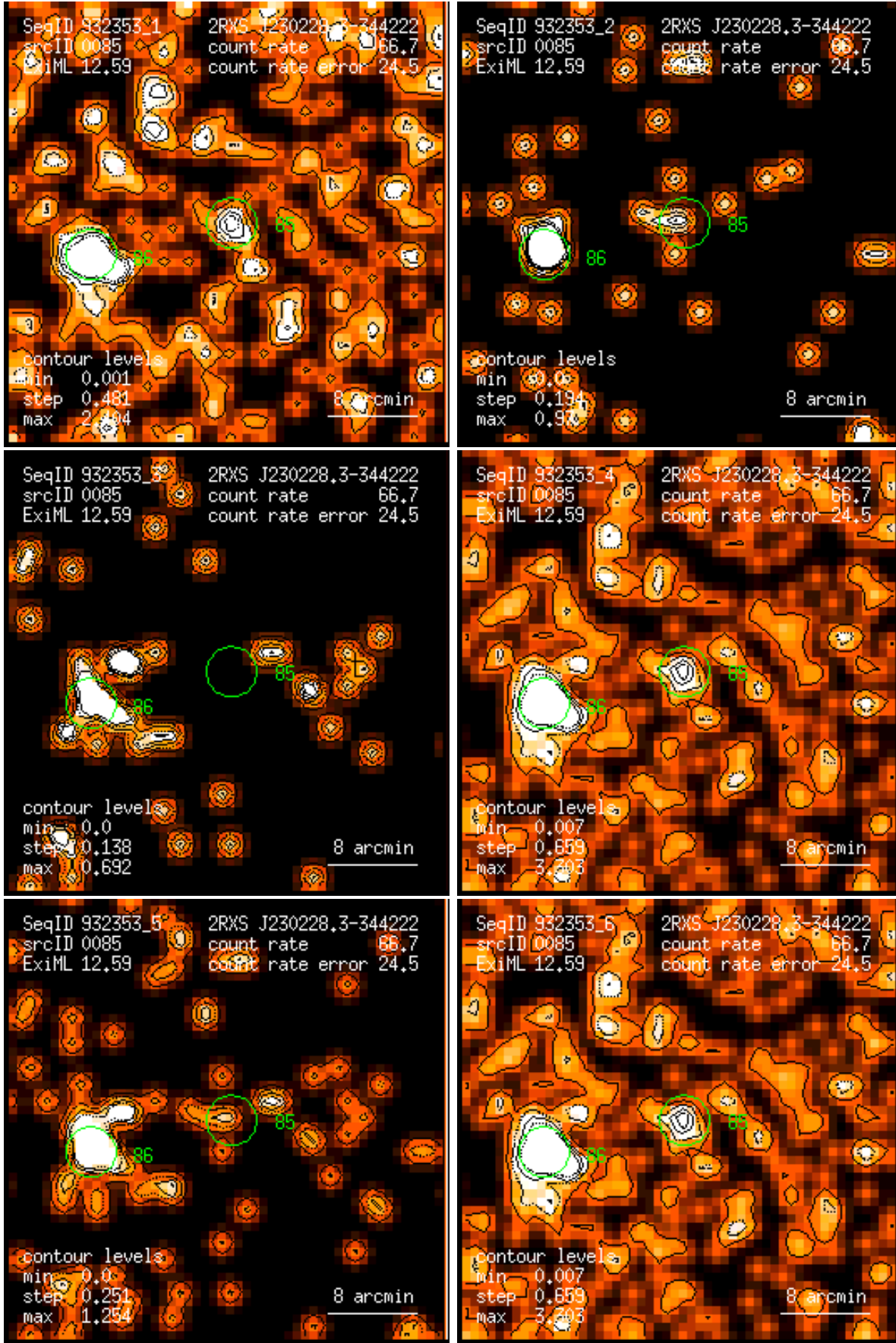
Figure 85: RASS 932353: detection 0085: band rate images, Gaussian filter: (1) PSPC channels 11 – 41, (2) 52 – 90, (3) 91 – 201, (4) 11 – 235, (5) 52 – 201, (6) 11 – 201. Broad band rates in counts/ks. Band rate contour levels in counts/ks/arcmin 2 .
