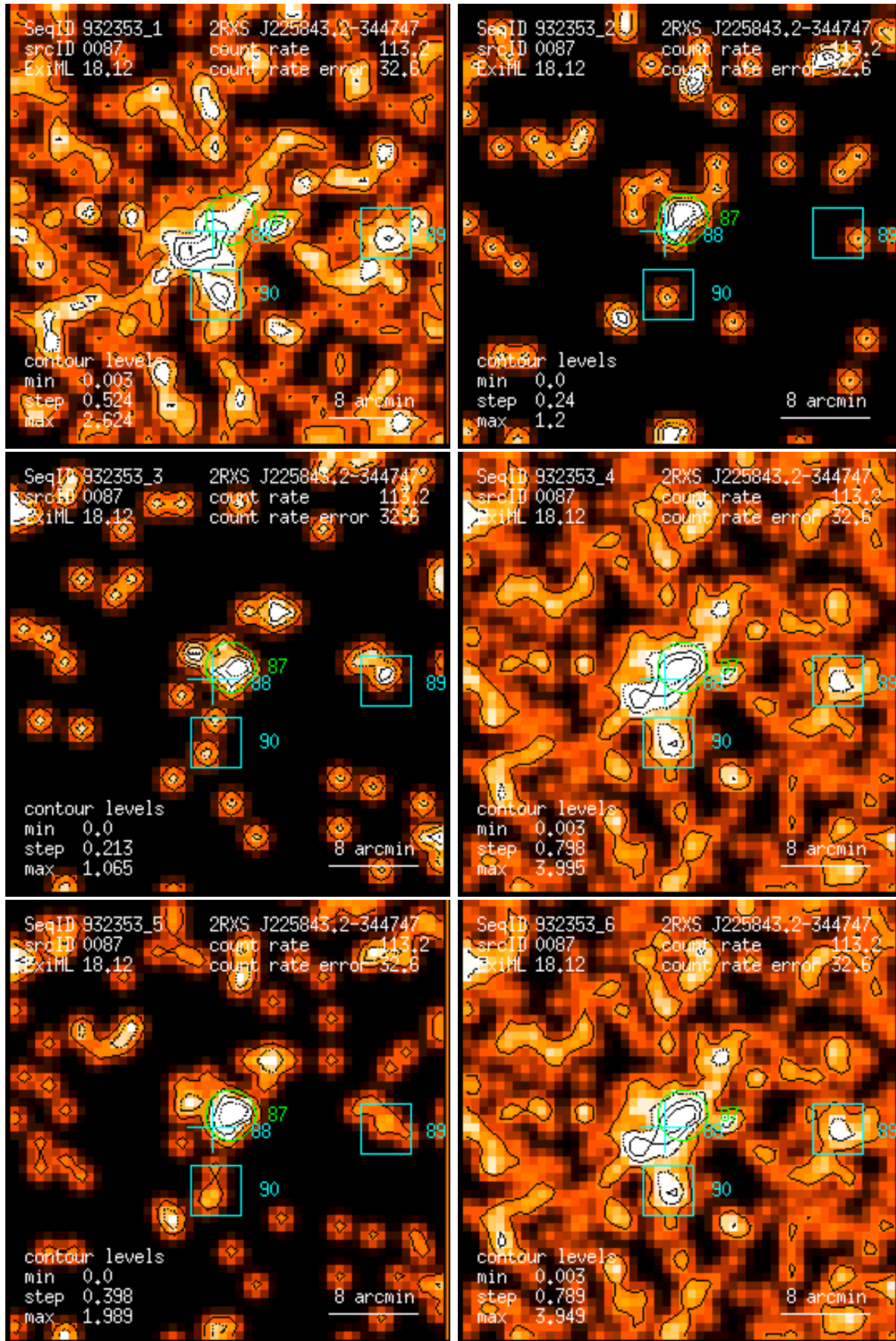
Figure 87: RASS 932353: detection 0087: band rate images, Gaussian filter: (1) PSPC channels 11 – 41, (2) 52 – 90, (3) 91 – 201, (4) 11 – 235, (5) 52 – 201, (6) 11 – 201. Broad band rates in counts/ks. Band rate contour levels in counts/ks/arcmin 2 .
