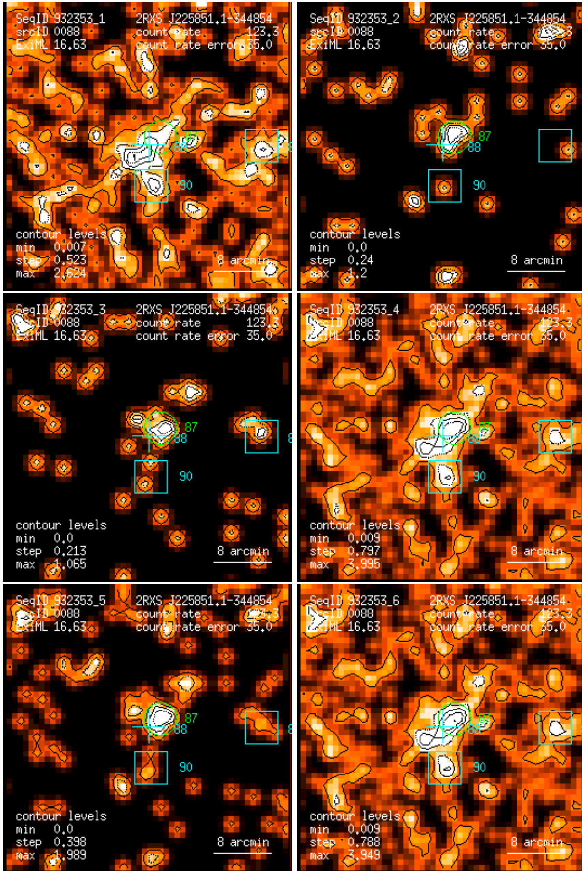
Figure 88: RASS 932353: detection 0088: band rate images, Gaussian filter: (1) PSPC channels 11 – 41, (2) 52 – 90, (3) 91 – 201, (4) 11 – 235, (5) 52 – 201, (6) 11 – 201. Broad band rates in counts/ks. Band rate contour levels in counts/ks/arcmin 2 .
