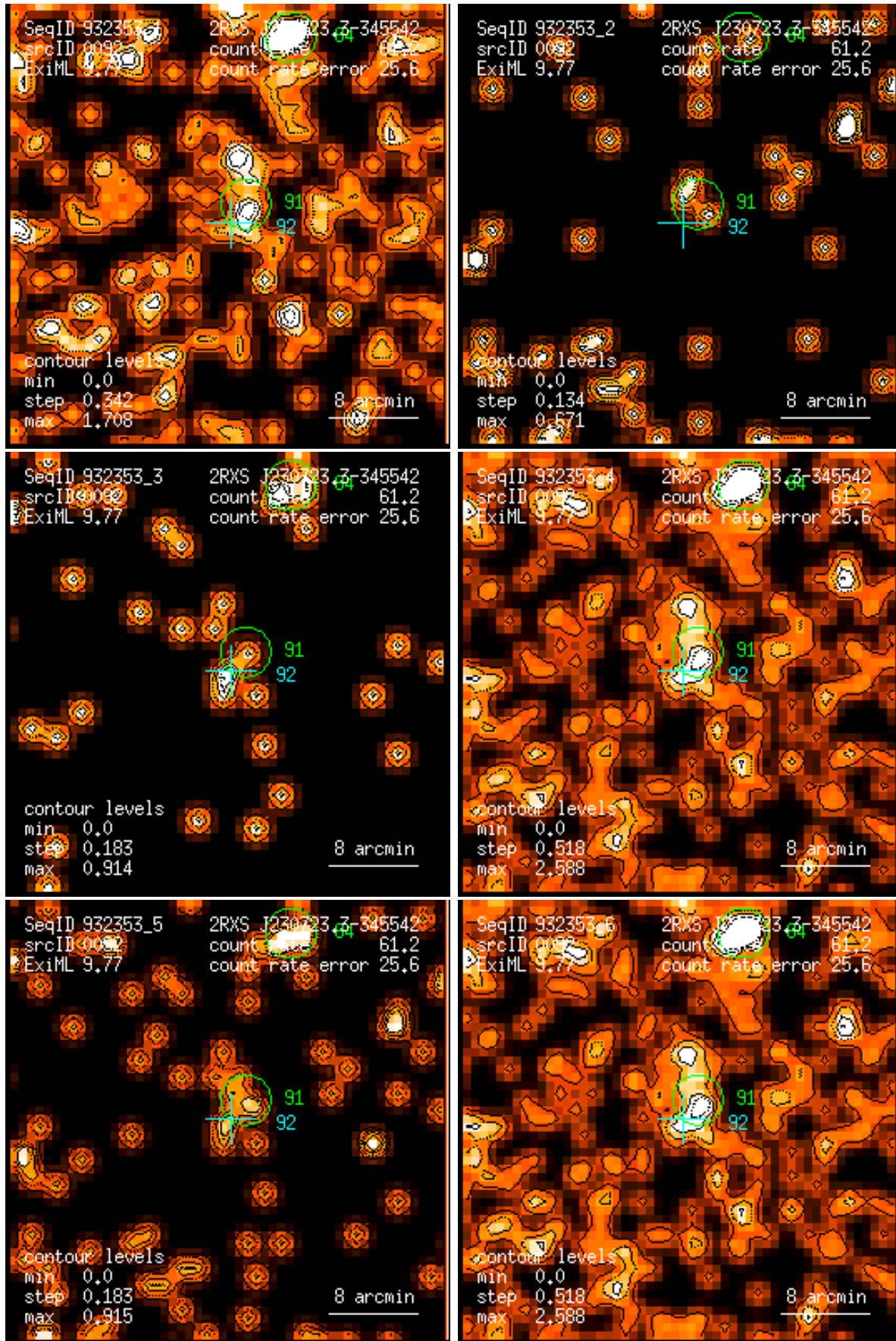
Figure 92: RASS 932353: detection 0092: band rate images, Gaussian filter: (1) PSPC channels 11 – 41, (2) 52 – 90, (3) 91 – 201, (4) 11 – 235, (5) 52 – 201, (6) 11 – 201. Broad band rates in counts/ks. Band rate contour levels in counts/ks/arcmin 2 .
