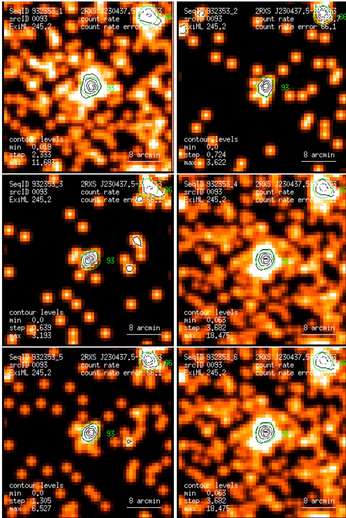
Figure 93: RASS 932353: detection 0093: band rate images, Gaussian filter: (1) PSPC channels 11 – 41, (2) 52 – 90, (3) 91 – 201, (4) 11 – 235, (5) 52 – 201, (6) 11 – 201. Broad band rates in counts/ks. Band rate contour levels in counts/ks/arcmin 2 .
