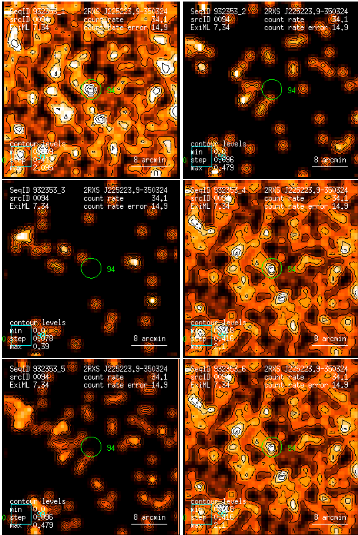
Figure 94: RASS 932353: detection 0094: band rate images, Gaussian filter: (1) PSPC channels 11 – 41, (2) 52 – 90, (3) 91 – 201, (4) 11 – 235, (5) 52 – 201, (6) 11 – 201. Broad band rates in counts/ks. Band rate contour levels in counts/ks/arcmin 2 .
