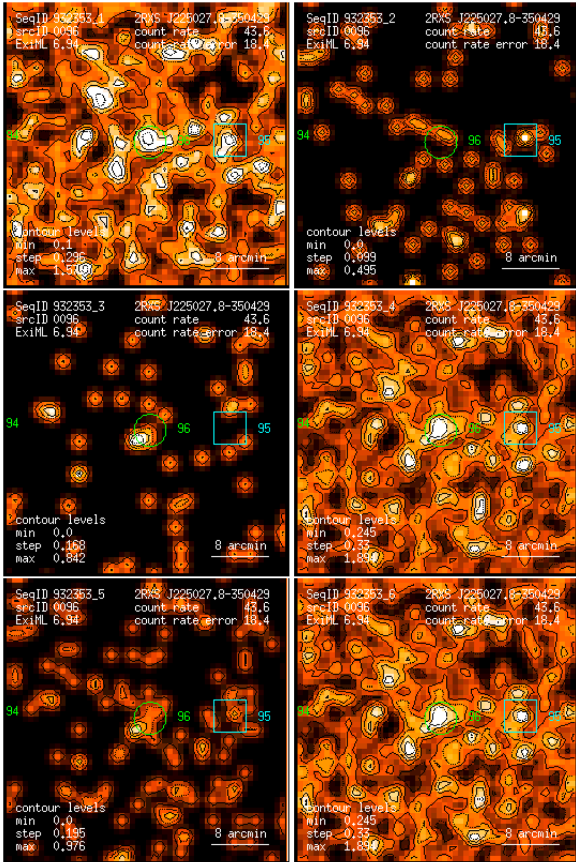
Figure 96: RASS 932353: detection 0096: band rate images, Gaussian filter: (1) PSPC channels 11 – 41, (2) 52 – 90, (3) 91 – 201, (4) 11 – 235, (5) 52 – 201, (6) 11 – 201. Broad band rates in counts/ks. Band rate contour levels in counts/ks/arcmin 2 .
