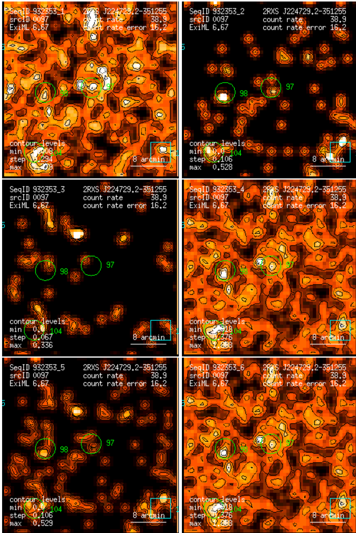
Figure 97: RASS 932353: detection 0097: band rate images, Gaussian filter: (1) PSPC channels 11 – 41, (2) 52 – 90, (3) 91 – 201, (4) 11 – 235, (5) 52 – 201, (6) 11 – 201. Broad band rates in counts/ks. Band rate contour levels in counts/ks/arcmin 2 .
