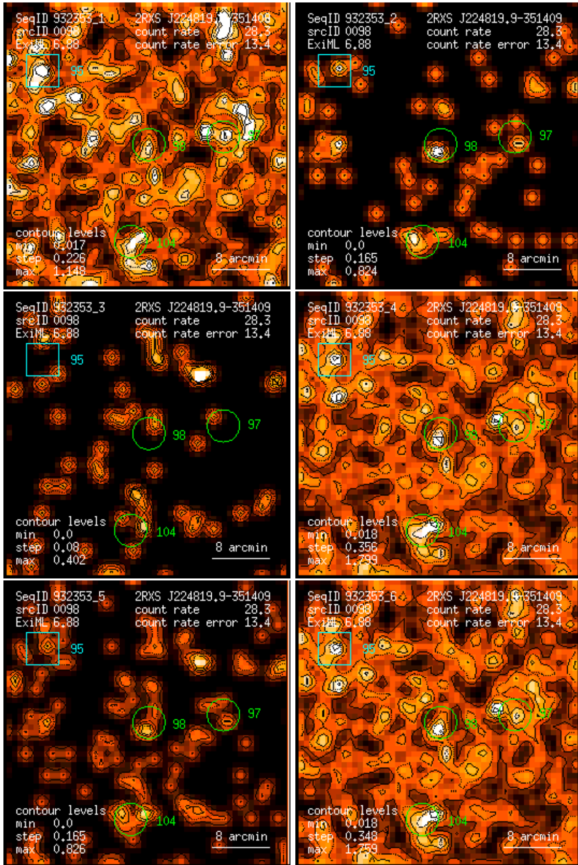
Figure 98: RASS 932353: detection 0098: band rate images, Gaussian filter: (1) PSPC channels 11 – 41, (2) 52 – 90, (3) 91 – 201, (4) 11 – 235, (5) 52 – 201, (6) 11 – 201. Broad band rates in counts/ks. Band rate contour levels in counts/ks/arcmin 2 .
