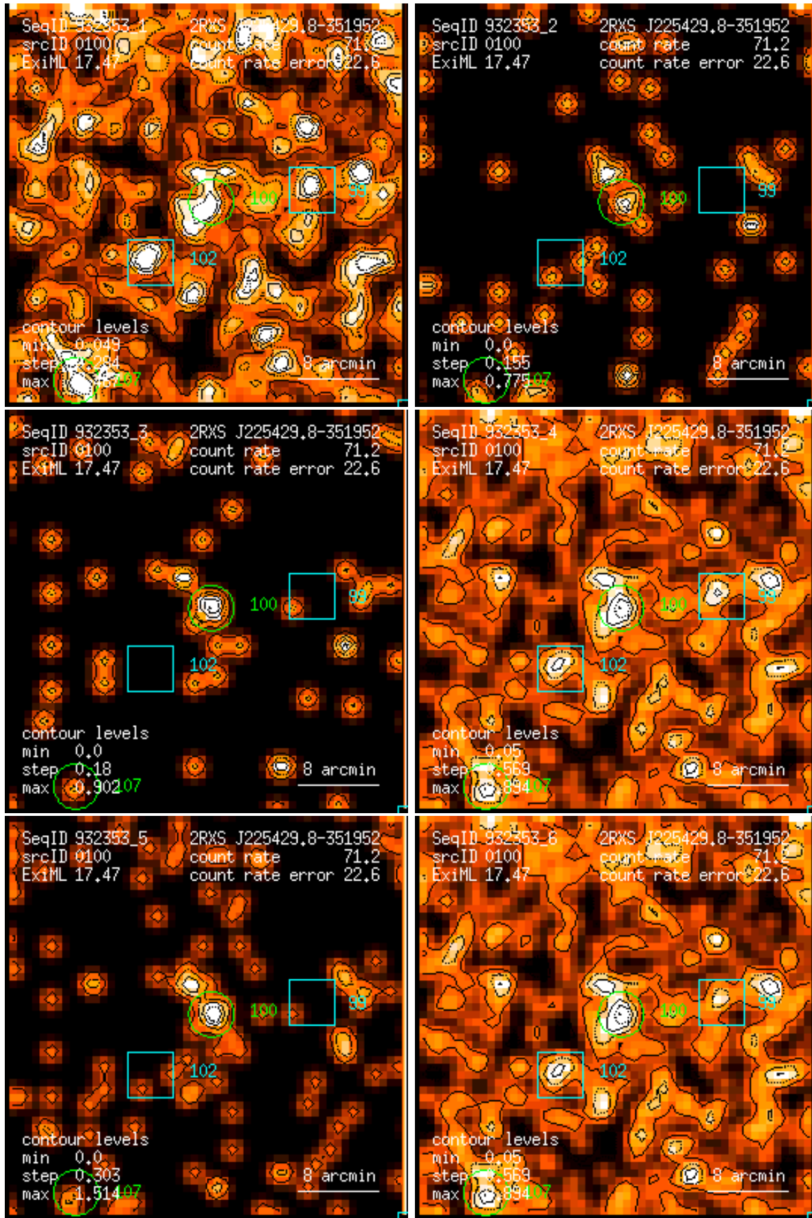
Figure 100: RASS 932353: detection 0100: band rate images, Gaussian filter: (1) PSPC channels 11 – 41, (2) 52 – 90, (3) 91 – 201, (4) 11 – 235, (5) 52 – 201, (6) 11 – 201. Broad band rates in counts/ks. Band rate contour levels in counts/ks/arcmin 2 .
