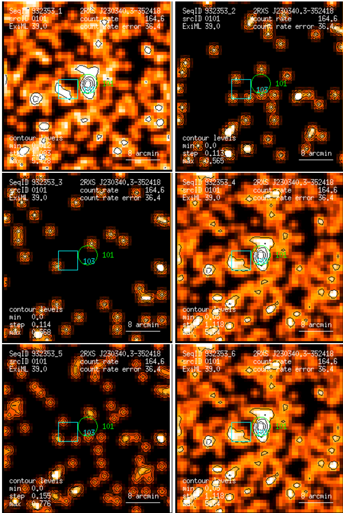
Figure 101: RASS 932353: detection 0101: band rate images, Gaussian filter: (1) PSPC channels 11 – 41, (2) 52 – 90, (3) 91 – 201, (4) 11 – 235, (5) 52 – 201, (6) 11 – 201. Broad band rates in counts/ks. Band rate contour levels in counts/ks/arcmin 2 .
