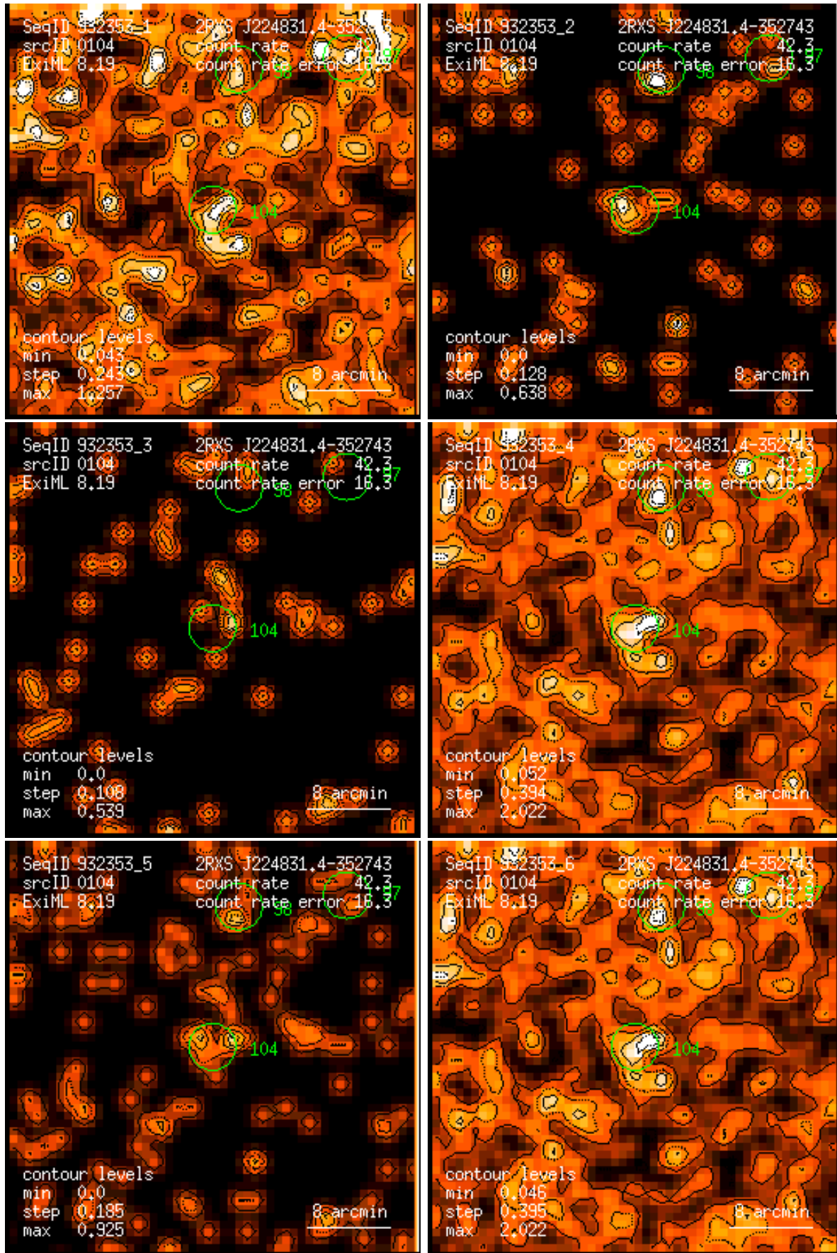
Figure 104: RASS 932353: detection 0104: band rate images, Gaussian filter: (1) PSPC channels 11 – 41, (2) 52 – 90, (3) 91 – 201, (4) 11 – 235, (5) 52 – 201, (6) 11 – 201. Broad band rates in counts/ks. Band rate contour levels in counts/ks/arcmin 2 .
